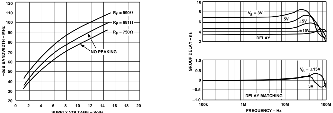
Figure 48. -3 dB Bandwidth vs. Supply Voltage for Gain = +2, R_L = 150 \Omega
