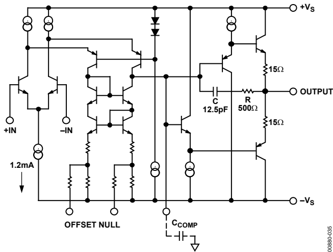
Figure 35. Simplified Schematic
