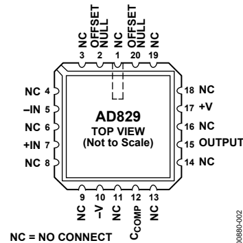
Figure 2. 20-Terminal LCC
