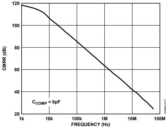
Figure 17. Common-Mode Rejection Ratio (CMRR) vs. Frequency
