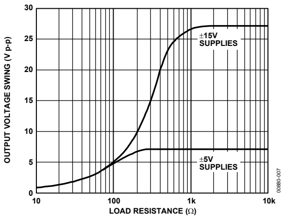
Figure 7. Output Voltage Swing vs. Resistive Load
