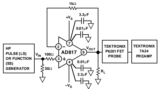
Figure 22. Noninverting Amplifier Connection
