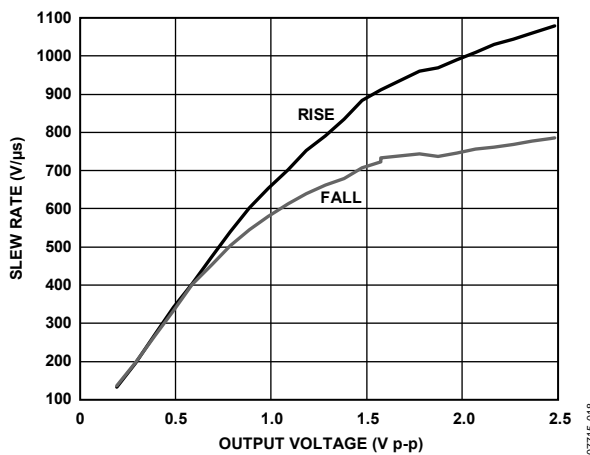
Figure 18. Slew Rate vs. Output Voltage
