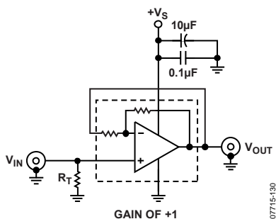
Figure 32. Unity Gain of Option 1
