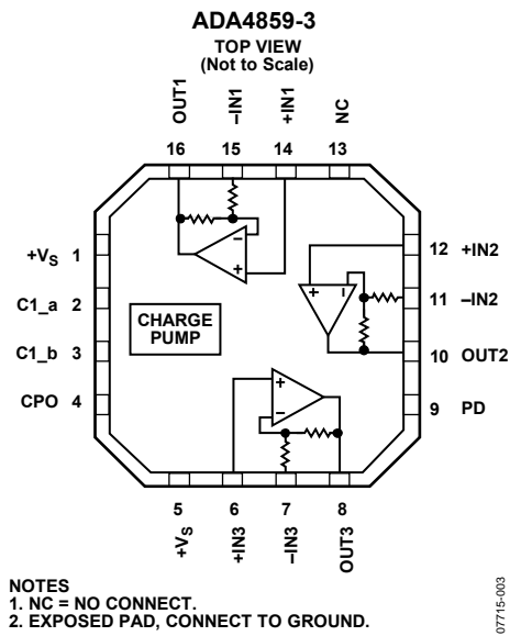
Figure 3. Pin Configuration
