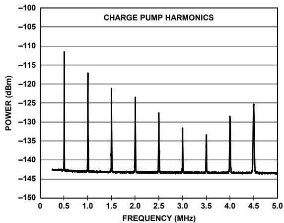
Figure 28. Output Spectrum vs. Frequency
