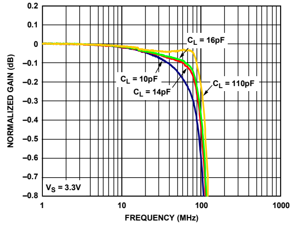
Figure 13. Large Signal 0.1 dB Flatness vs. Capacitive Load
