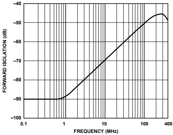
Figure 11. Forward Isolation vs. Frequency
