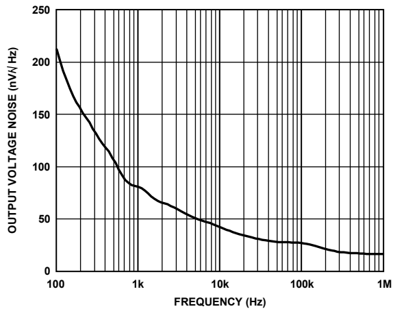
Figure 12. Total Output Voltage Noise vs. Frequency
