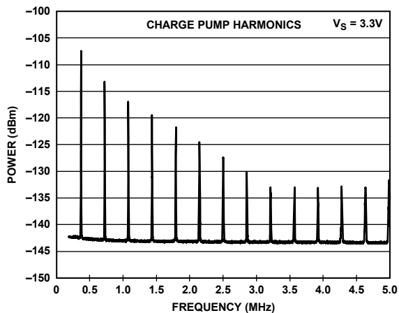
Figure 29. Output Spectrum vs. Frequency
