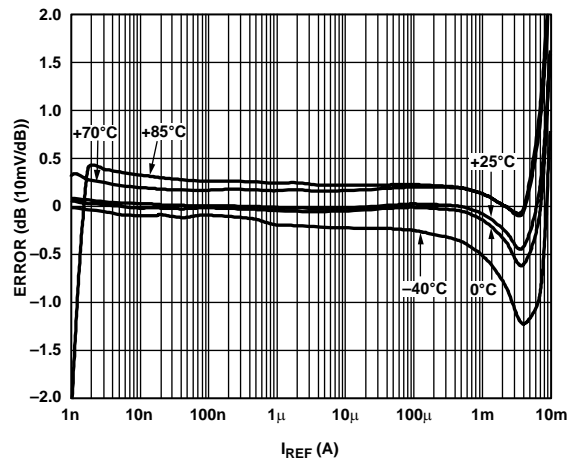
Figure 7. Law Conformance Error vs. I_{REF} for Multiple Temperatures, Normalized to 25°C ( I_{INP} = 3\text{ }\mu\text{A} )
