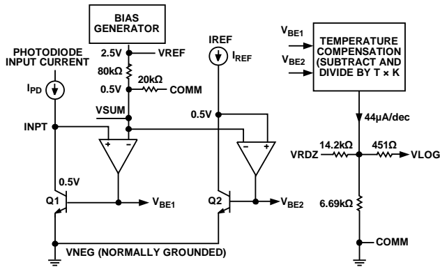
Figure 33. Simplified Schematic
