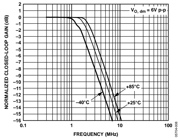
Figure 9. Large Signal Frequency Response at Various Temperatures
