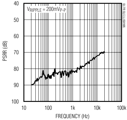
POWER-SUPPLY REJECTION RATIO vs. FREQUENCY (SPEAKER MODE)
