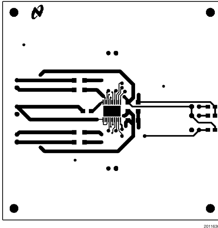
FIGURE 3. Recommended MH PC Board Layout: Component-Side Layout
