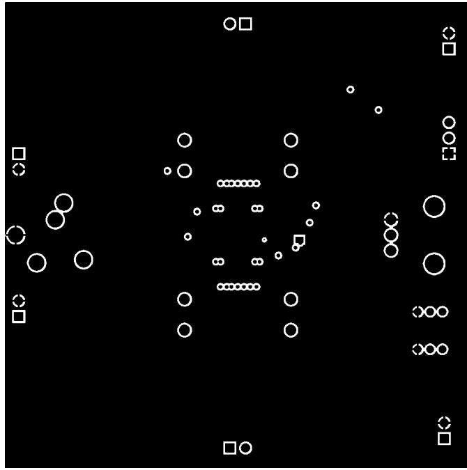
FIGURE 6. Bottom Layer
