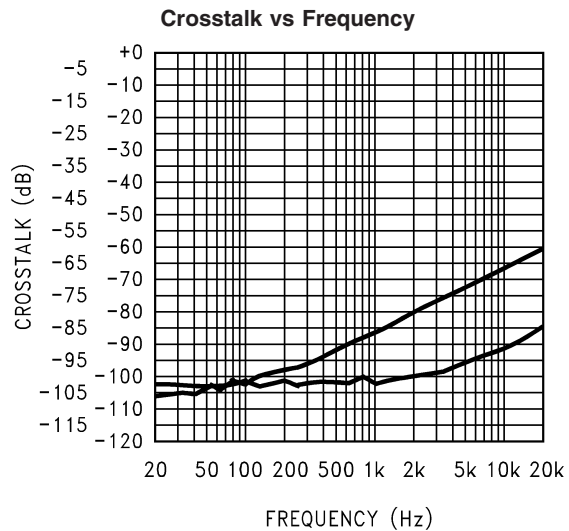
20079735 V DD = 3V; LLS, RLS; P O = 200mW; R L = 8Ω; Mode 7; 0db Gain; 3D off Top-Left to Right; Bot- Right to Left
