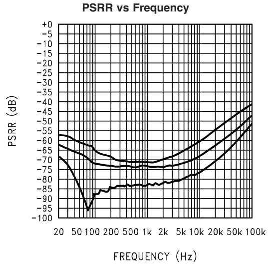
20079733 V DD = 3V; LINEOUT; R L = 5kΩ; 0db Gain; All audio inputs terminated Top-Mode 15; Mid-Mode 10; Bot-Mode 5
