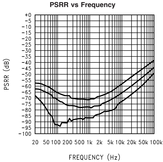
20079732 V DD = 5V; LINEOUT; R L = 5kΩ; 0db Gain; All audio inputs terminated Top-Mode 15; Mid-Mode 10; Bot-Mode 5
