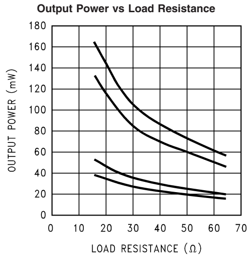
LHP, RHP; R_L = 32\Omega ; Top- V_{DD} = 5V , 10% THD+N; Topmid- V_{DD} = 5V , 1% THD+N; Botmid- V_{DD} = 3V , 10% THD+N; Bot- V_{DD} = 3V , 1% THD+N
