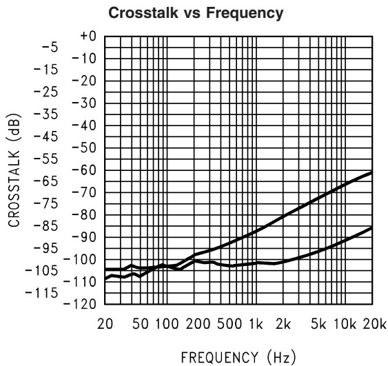
20079734 V DD = 5V; LLS, RLS; P O = 400mW; R L = 8Ω; Mode 7; 0db Gain; 3D off Top-Left to Right; Bot- Right to Left
