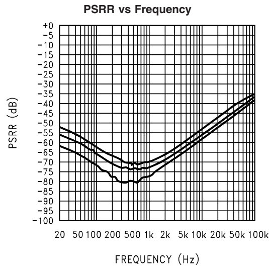
V_{DD} = 3V ; EP; R_L = 32\Omega ; 0db Gain; All audio inputs terminated Top-Mode 11; Mid-Mode 6; Bot-Mode 1
