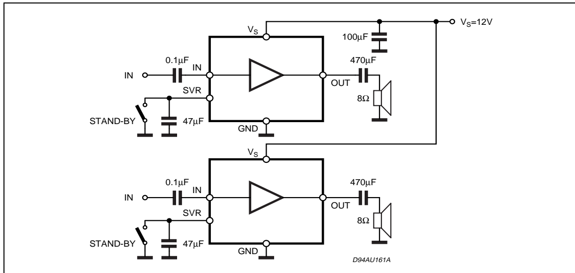
Figure 1. Application Circuit
