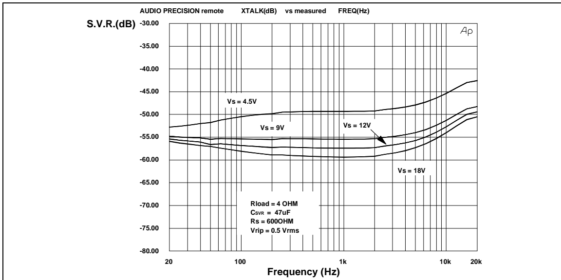
Figure 5. SVR vs Frequency
