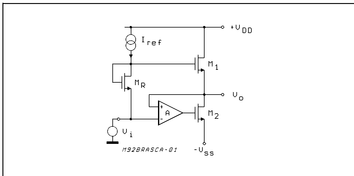
Figure 3: Principle Schematic of a DMOS unity-gain buffer.
