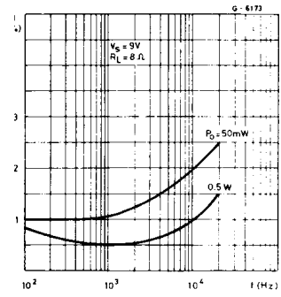
Figure 14. Distortion vs. frequency
