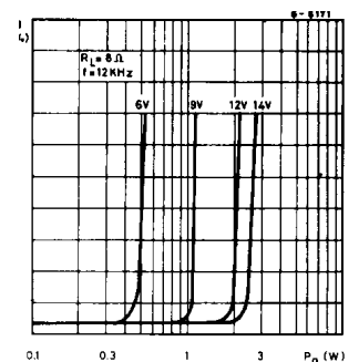
Figure 11. Distortion vs. output power
