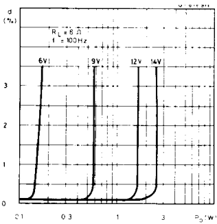
Figure 9. Distortion vs. output power
