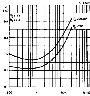
Figure 13. Distortion vs. frequency
