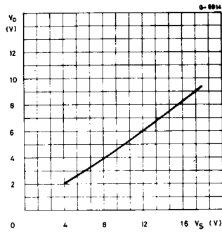
Figure 3. Quiescent output voltage vs. supply voltage
