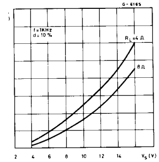
Figure 5. Output power vs. supply voltage
