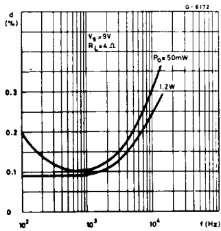
Figure 12. Distortion vs. frequency
