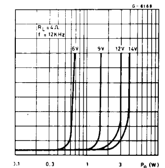
Figure 8. Distortion vs. output power
