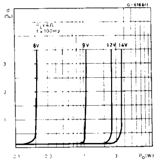
Figure 6. Distortion vs. output power
