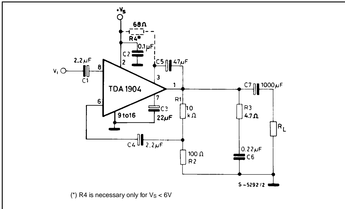
Figure 1. Test and application circuit
