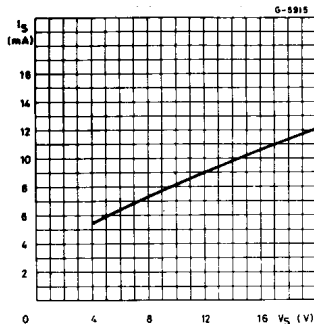
Figure 4. Quiescent drain current vs. supply voltage
