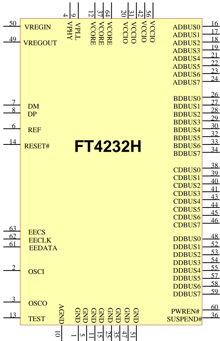
Figure 3.1 FT4232H Schematic Symbol
