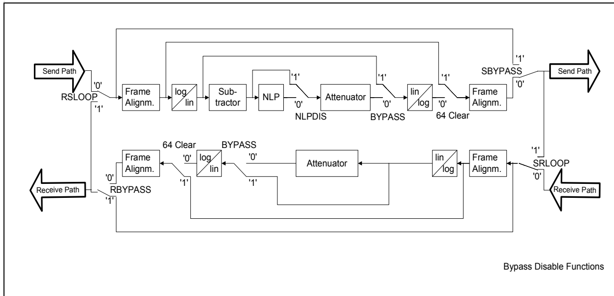
Figure 10 Bypass and Disabling Functions of the SIDE C
