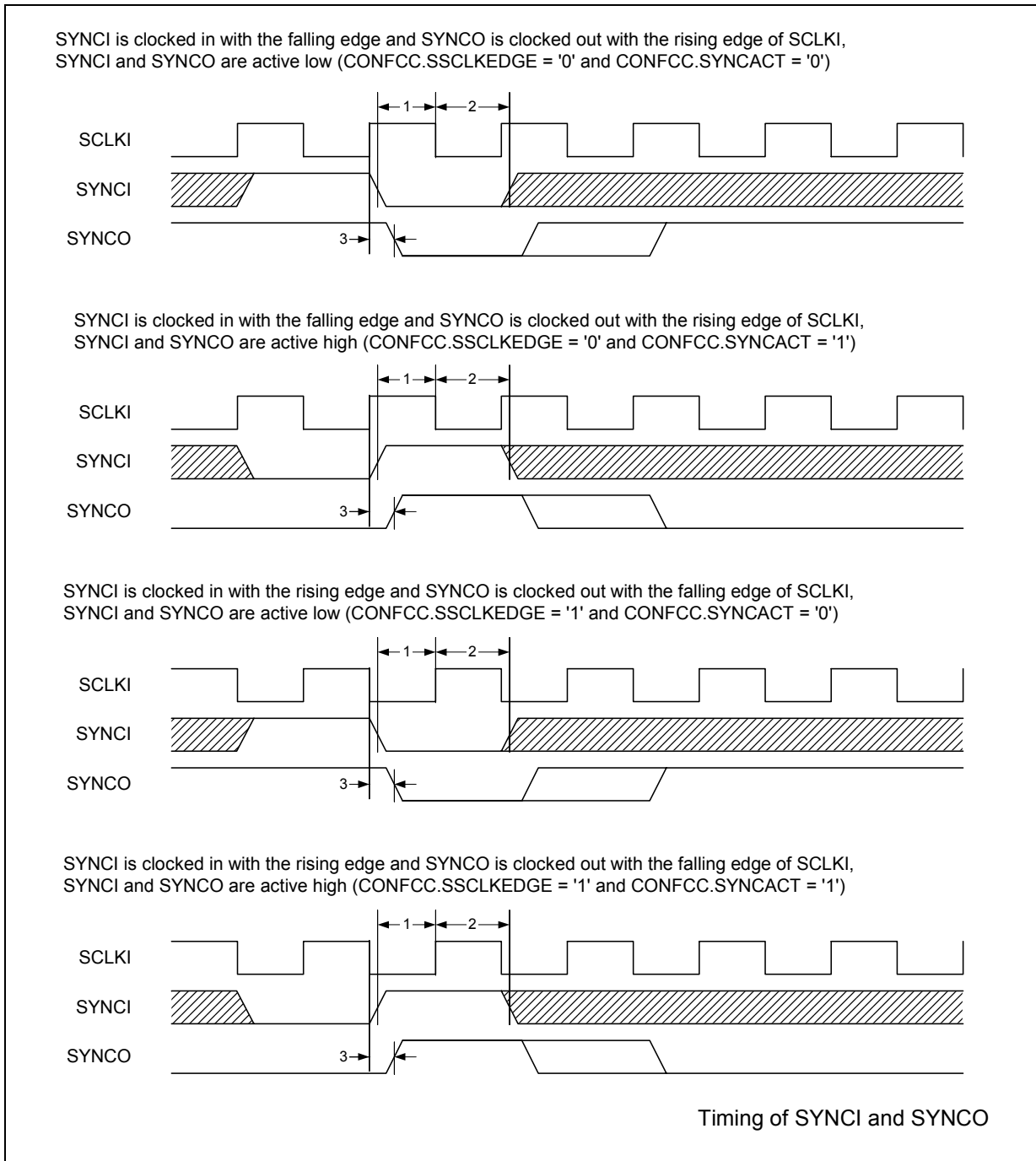
Figure 34 Timing of SYNCI and SYNCO
