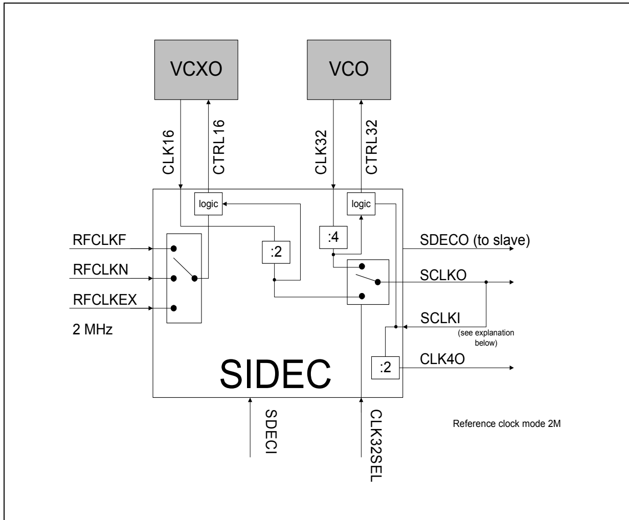
Figure 16 Reference Clock Mode with 2.048 MHz
