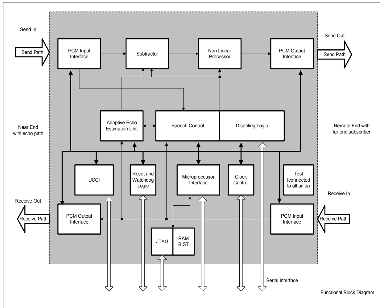
Figure 8 Block Diagram
