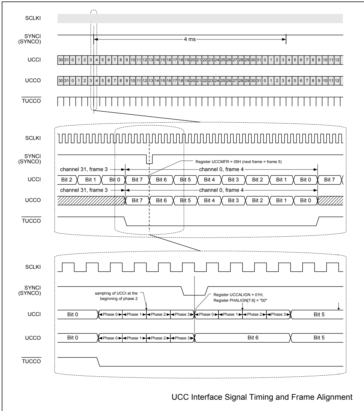
Figure 37 UCC Interface Signal Timing and Frame Alignment
