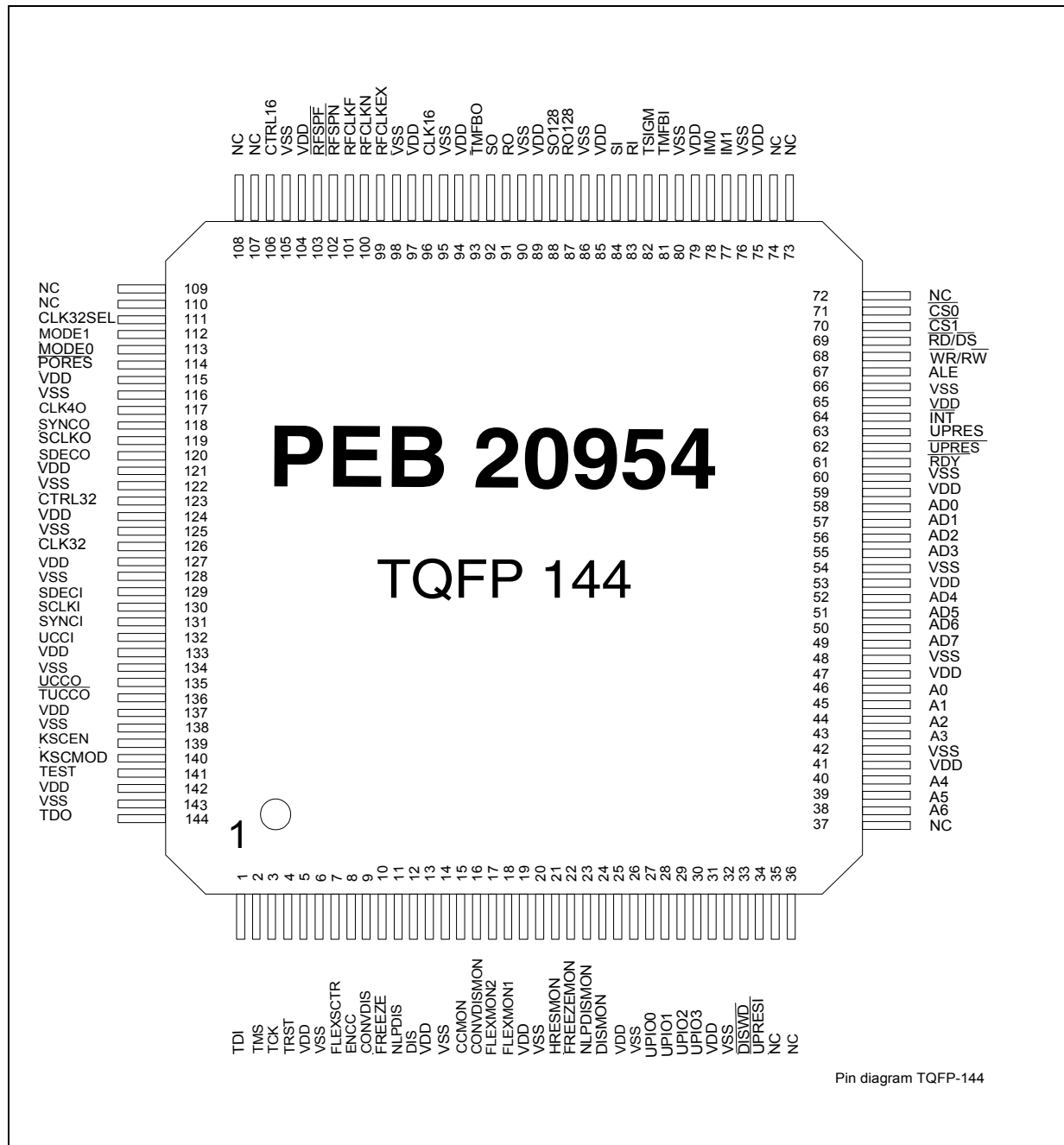
Figure 6 Pin Configuration P-TQFP-144-8
