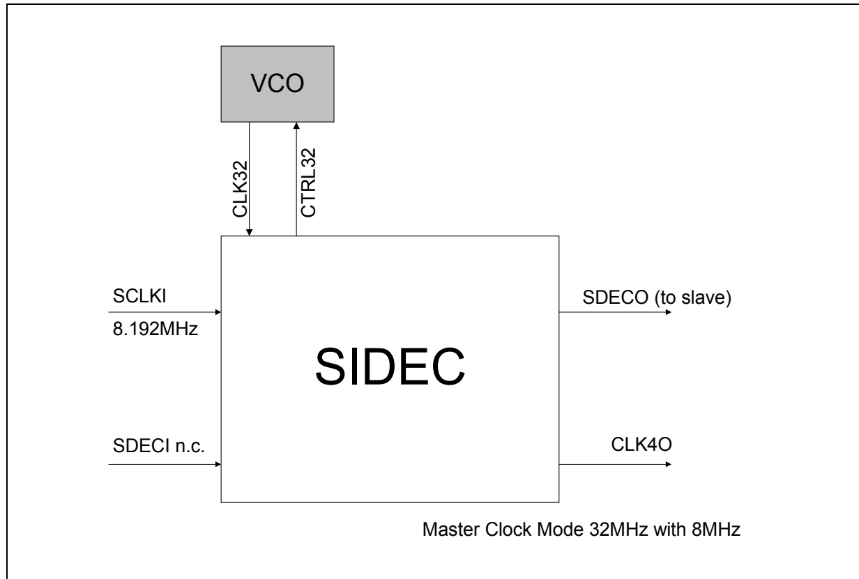
Figure 14 Master Clock Mode with External 8.192 MHz Clock
