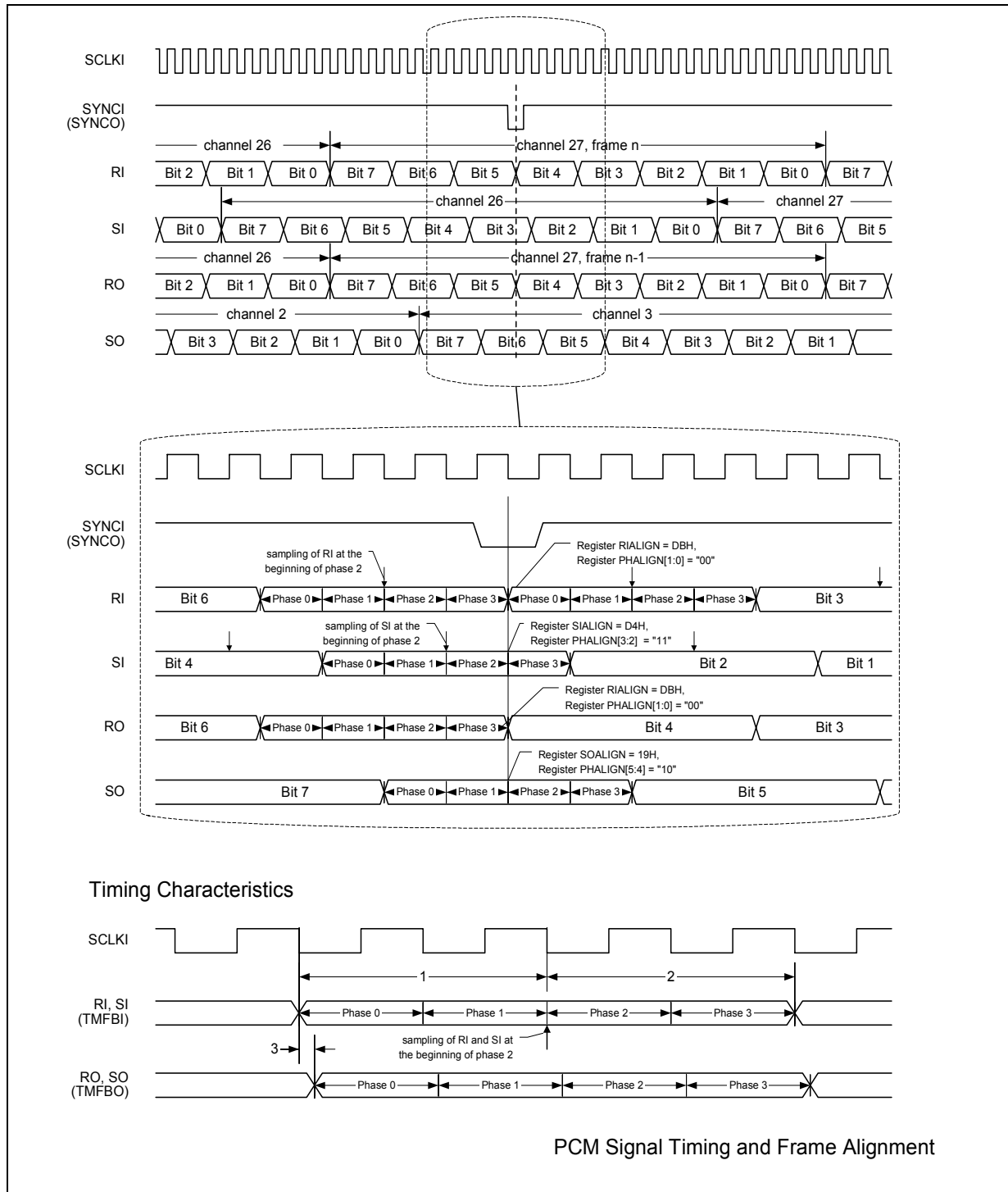
Figure 31 PCM Signal Timing and Frame Alignment
