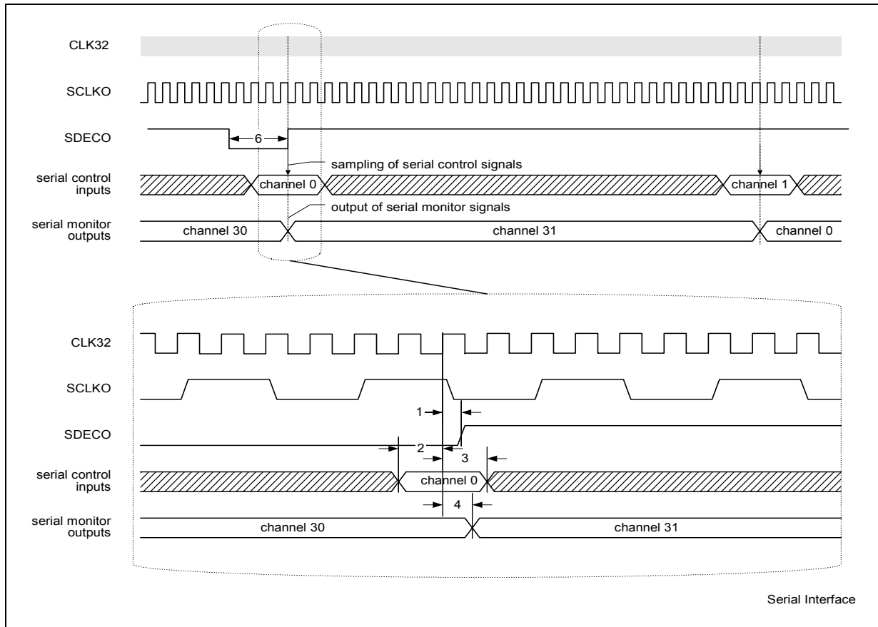
Figure 36 Serial Interface (Controlling and Monitoring) Timing
