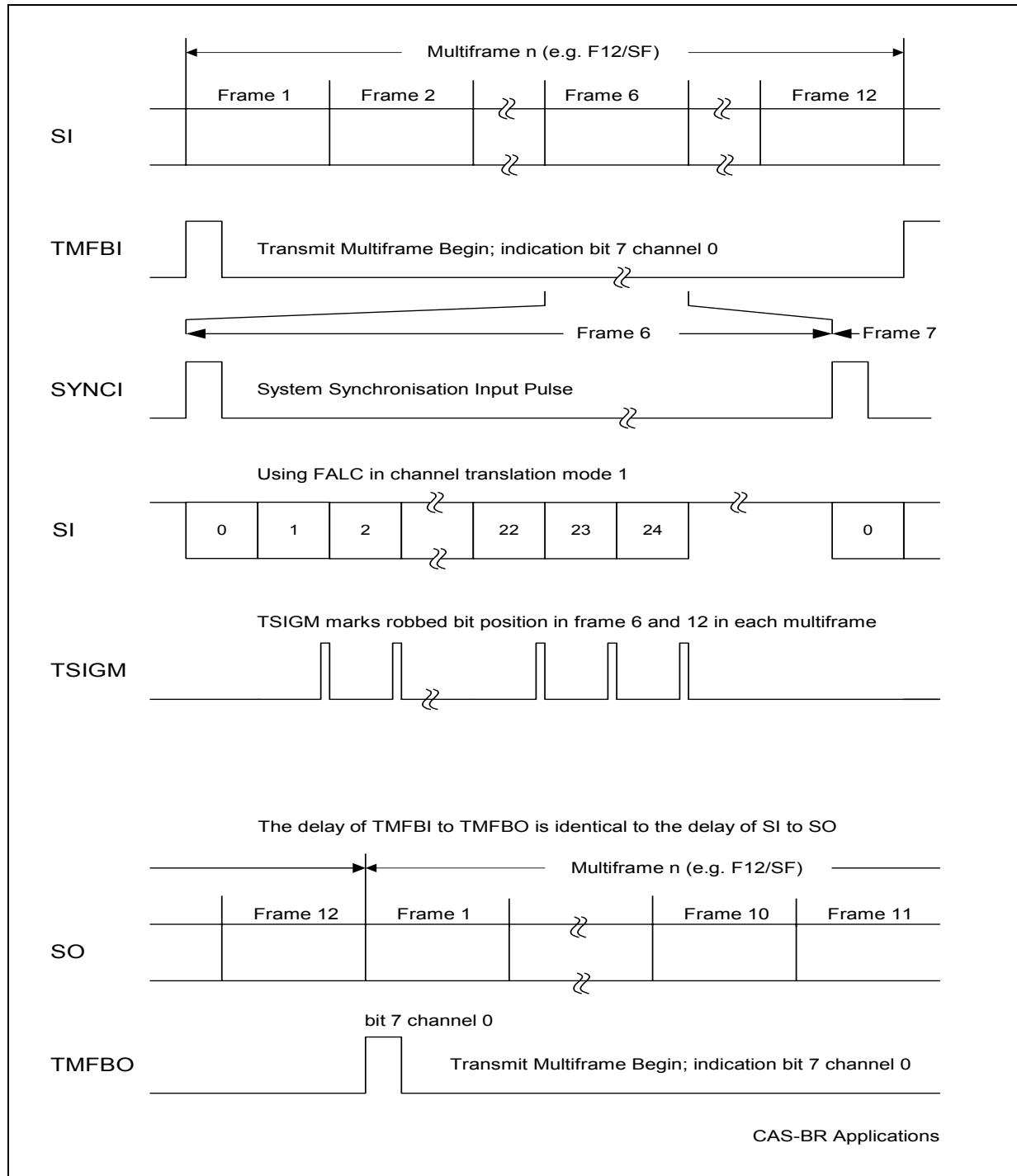
Figure 39 Timing of Supporting signals for CAS-BR Applications
