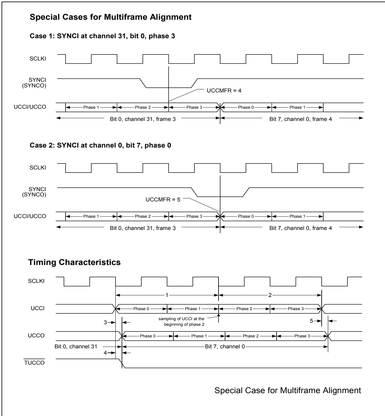
Figure 38 Special Cases for Multiframe Alignment and Timing Characteristics
