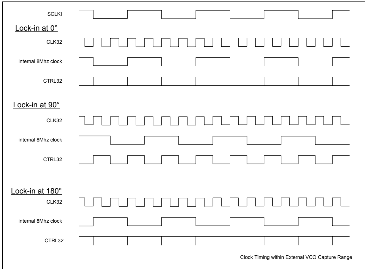
Figure 35 Clock Timing within External VCO Capture Range
