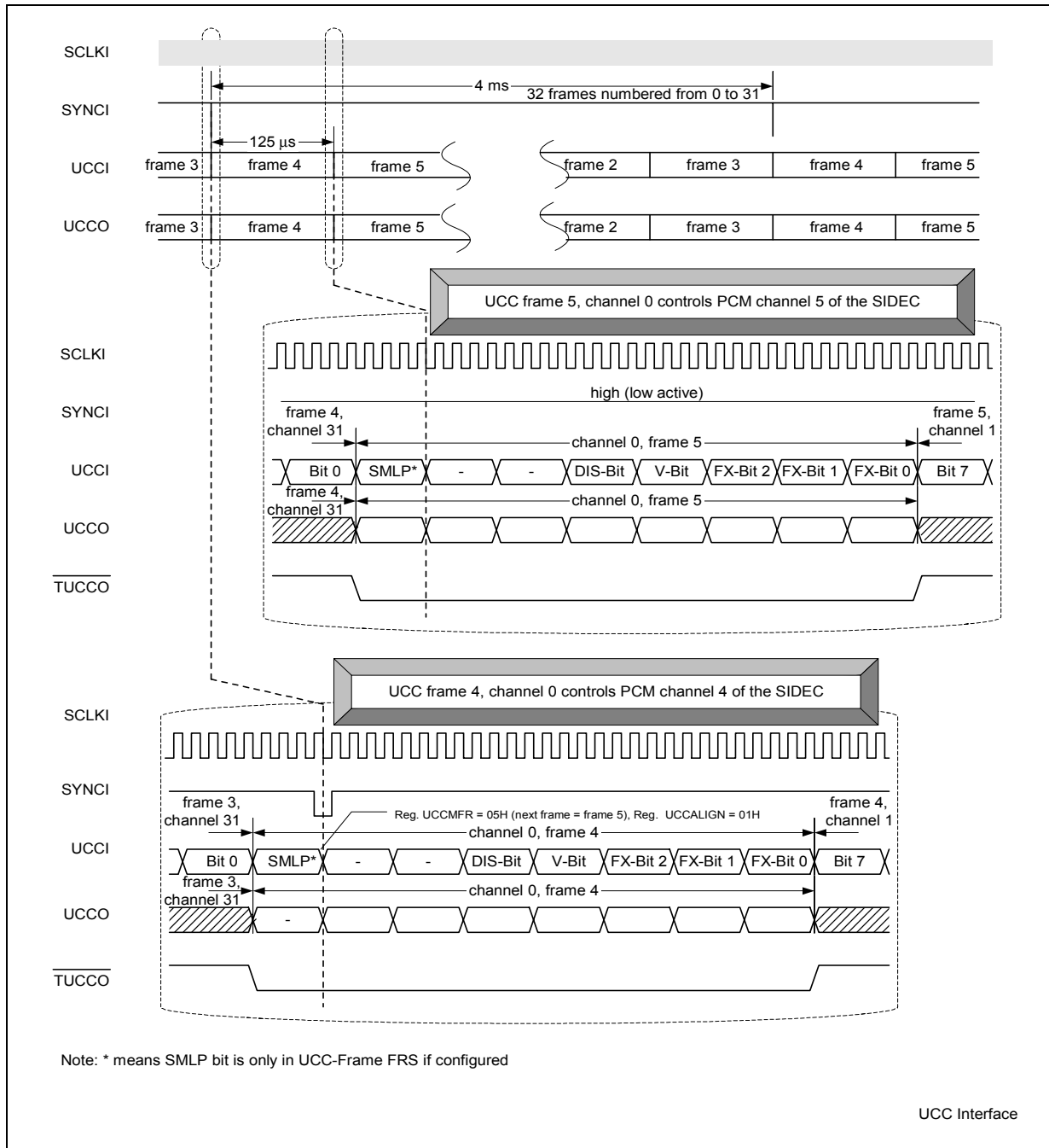
Figure 11 UCC Signal for control of PCM Signal
