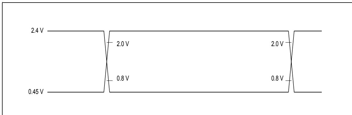
Figure 29 Input/Output Waveforms for AC-Tests
