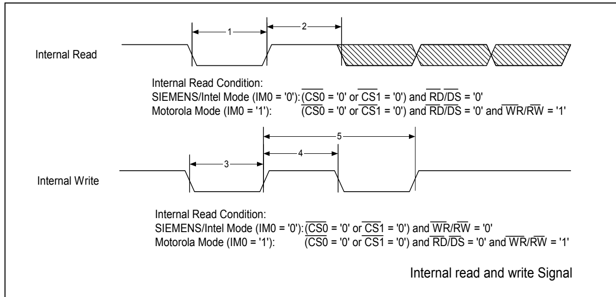
Figure 40 Internal Read Signal and Internal Write Signal
