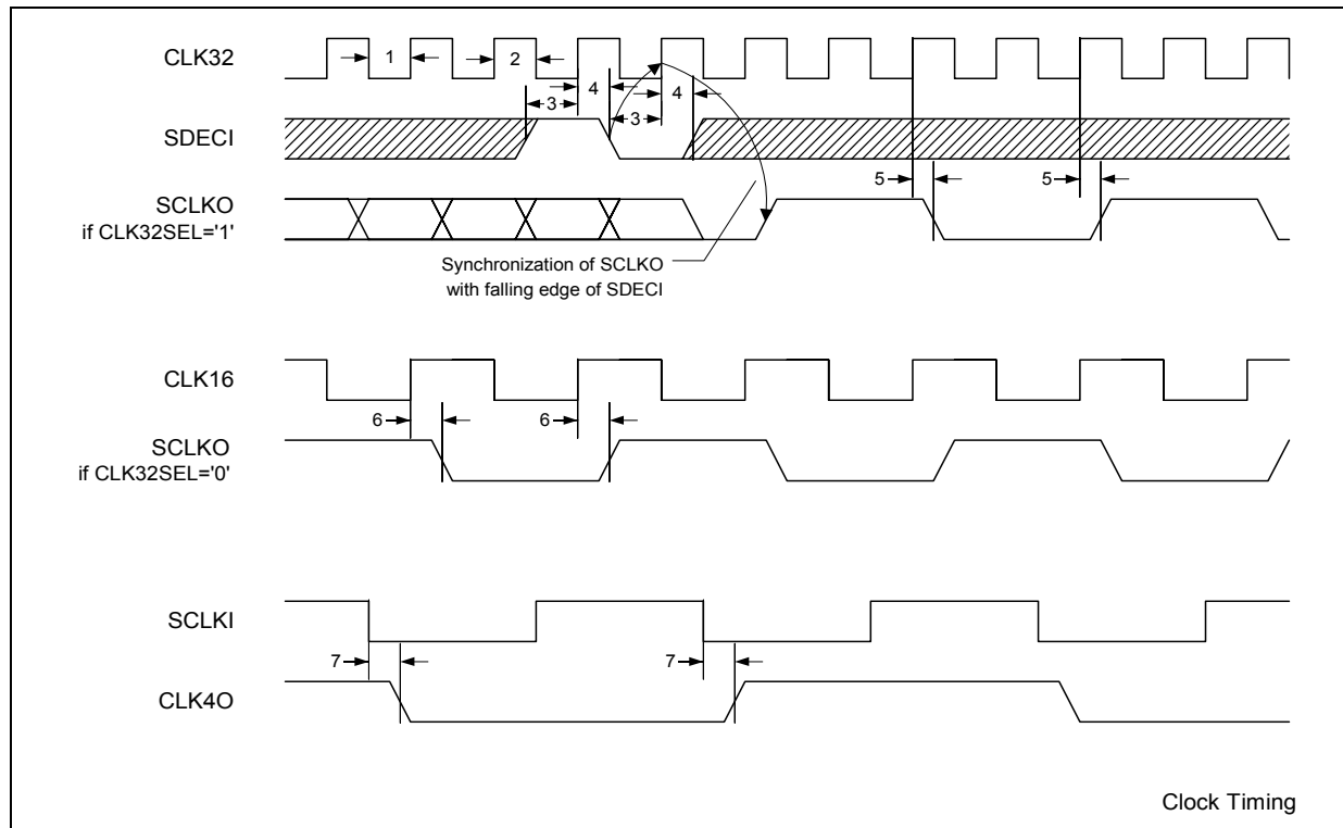
Figure 30 Clock Timing
