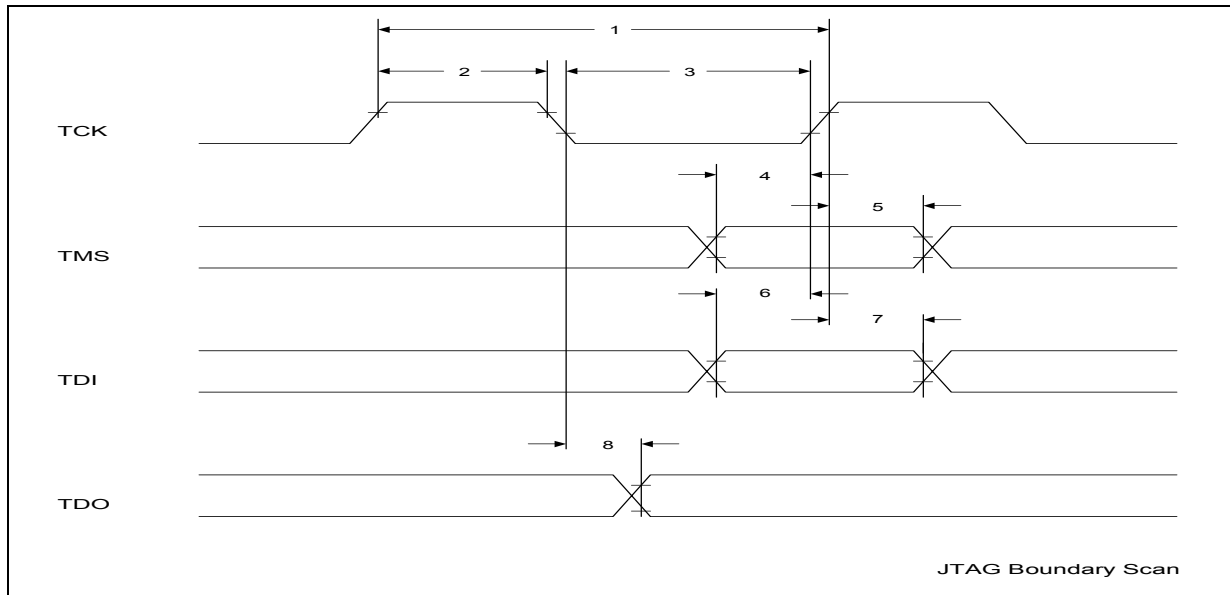
Figure 49 JTAG Boundary Scan Timing
