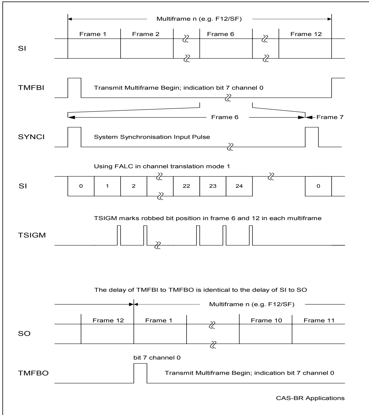
Figure 27 Timing of Supporting signals for CAS-BR Applications
