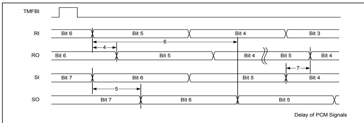
Figure 32 Delay of PCM Signals
