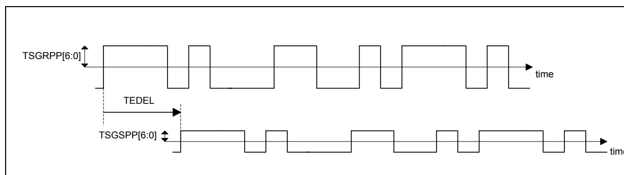
Figure 28 Explanation of Test Pattern Generation (random sign signal)
