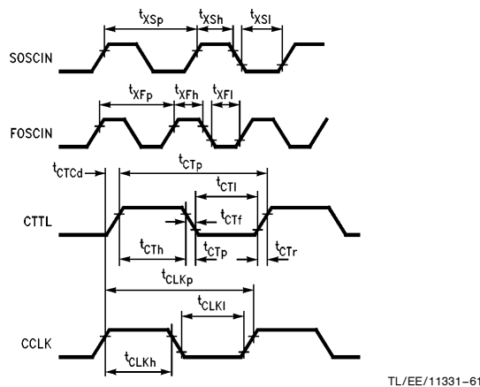
FIGURE 4-8. Clock Waveforms
