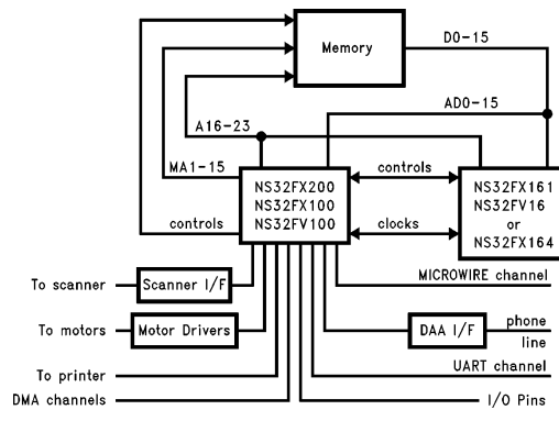
FIGURE 1-1. A FAX Controller Block Diagram
