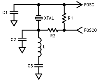
FIGURE 3-2. Oscillator Circuits
