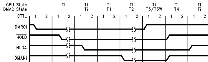
FIGURE 3-19. CPU/DMA Arbitration
