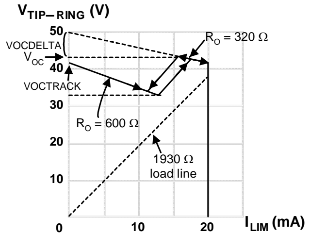
Figure 10. V_{TIP-RING} vs. I_{LOOP} Characteristics using Modfeed™
