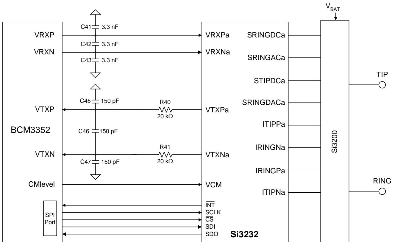
Figure 5. Typical Connection Diagram between Si3232 and Broadcom® BCM3352 (One SLIC channel shown: Channel “a”)
