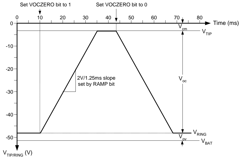
Figure 23. Wink Function with Programmable Ramp Rate
