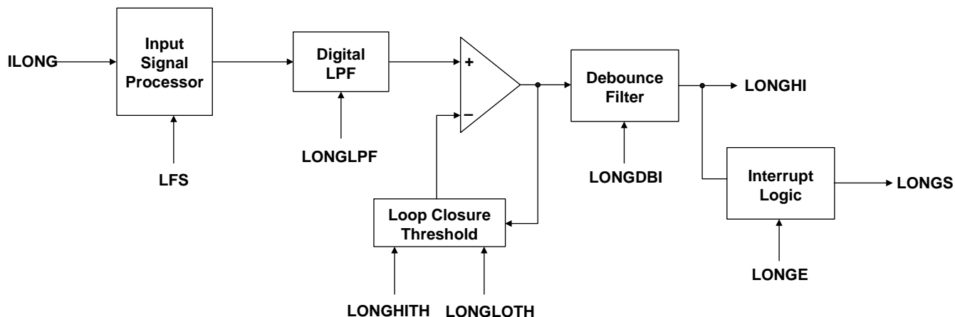
Figure 15. Ground Key Detection Circuitry
