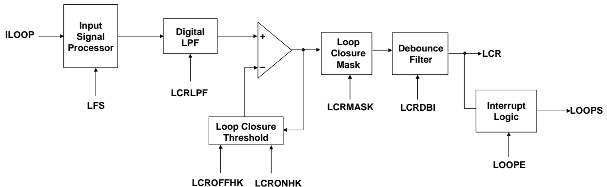
Figure 14. Loop Closure Detection Circuitry
