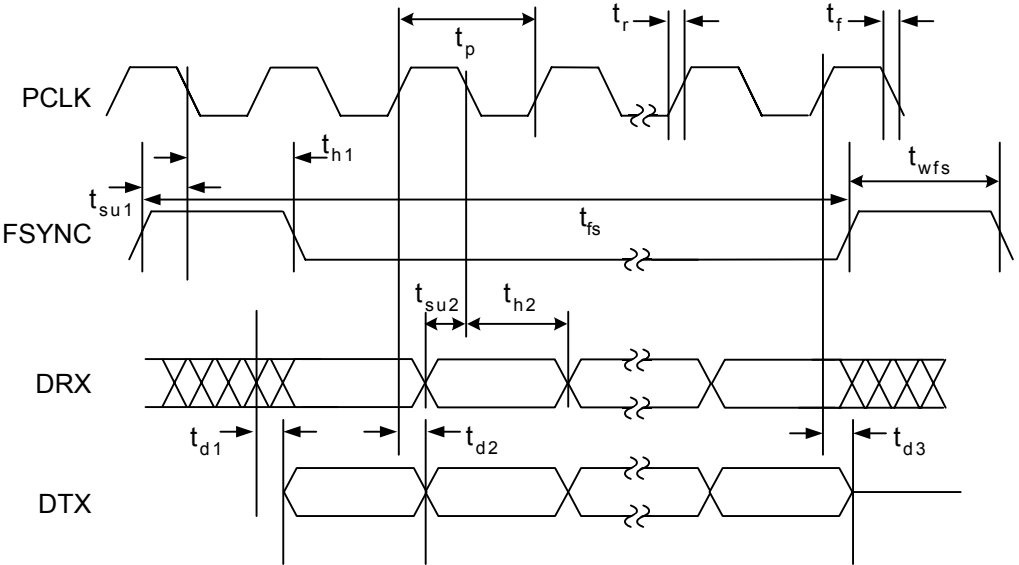
Figure 2. PCM Highway Interface Timing Diagram
