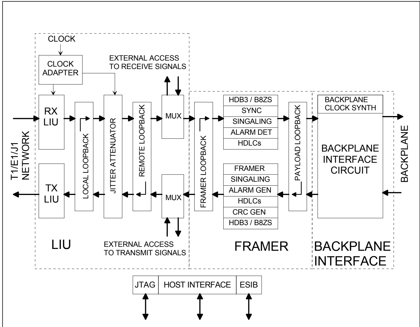
Figure 3-1. Block Diagram
