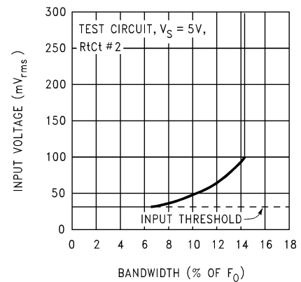
Bandwidth vs. Input Signal Level
