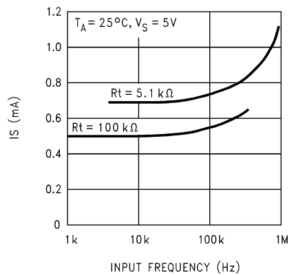
Supply Current vs. Operating Frequency
