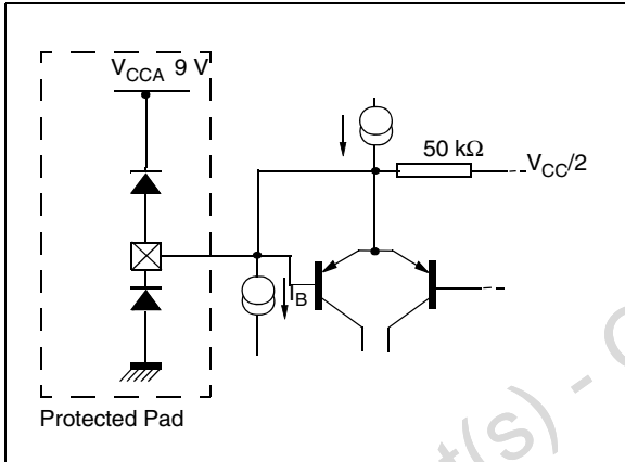
Figure 13. Audio inputs pins 11, 13, 19, 20, 22 and 23)
