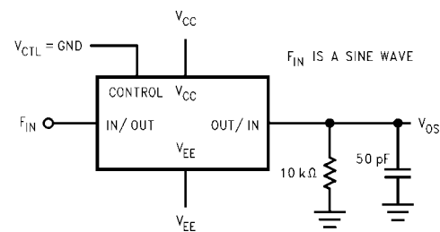
FIGURE 11. Sinewave Distortion
