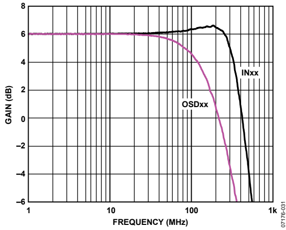
Figure 56. ADV3201 Small Signal Frequency Response, 200 mV p-p
