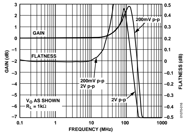
Figure 11. AD8115 Frequency Response, R_L = 1\ k\Omega
