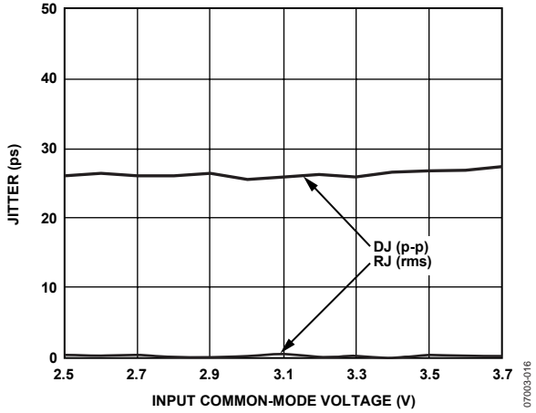
Figure 15. Jitter vs. Input Common-Mode Voltage
