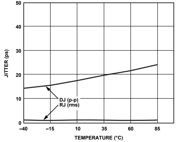
Figure 17. Jitter vs. Temperature
