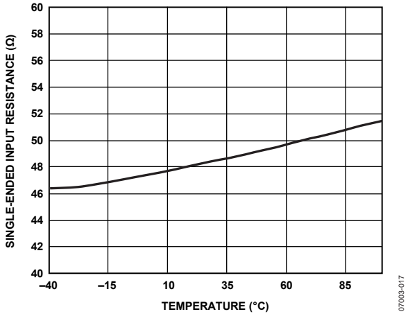
Figure 16. Single-Ended Input Resistance vs. Temperature
