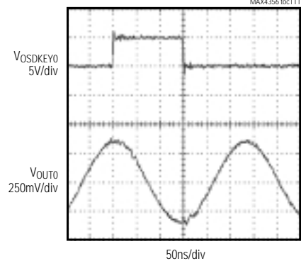
OSD SWITCHING 3.58MHz SIGNAL
