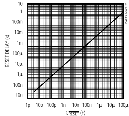
RESET DELAY vs. C RESET
