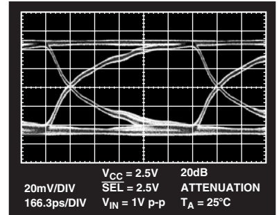
TPC 21. Eye Pattern; 1 Gbps, V_{CC} = 2.5V , PRBS 31
