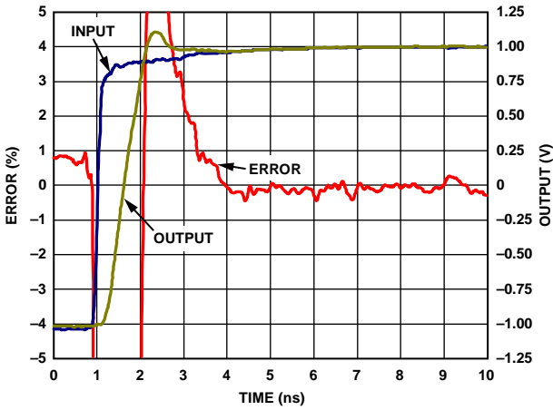
Figure 30. ADV3221 Settling Time, 2 V Step
