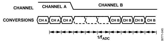
Figure 33. Sinc 3 Channel Change
