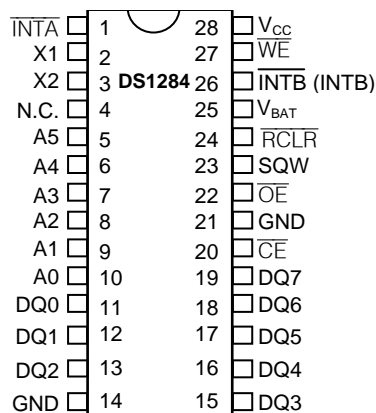
DIP (600 mils)
