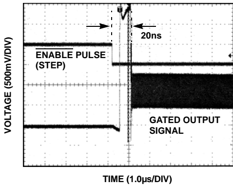
FIGURE 31. ENABLE TIME
