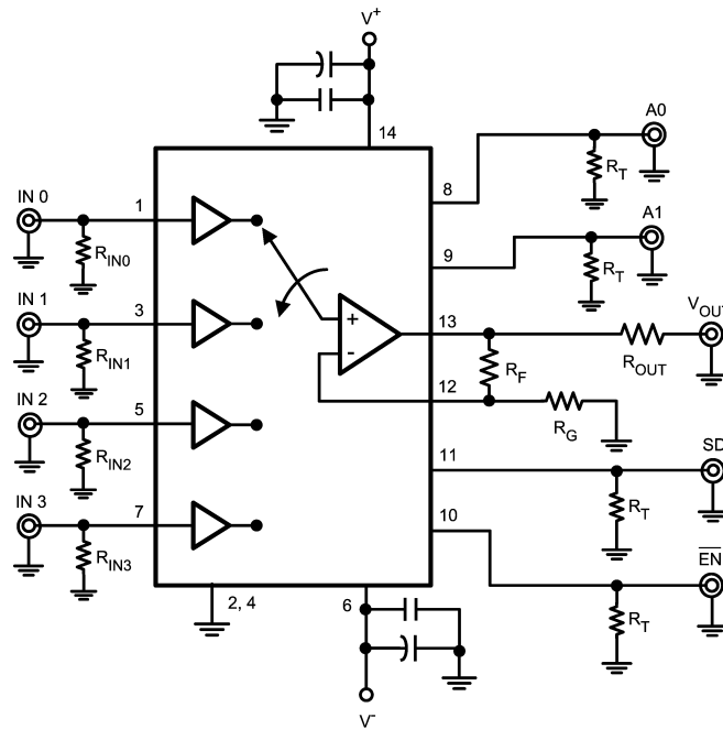
FIGURE 1. Typical Application
