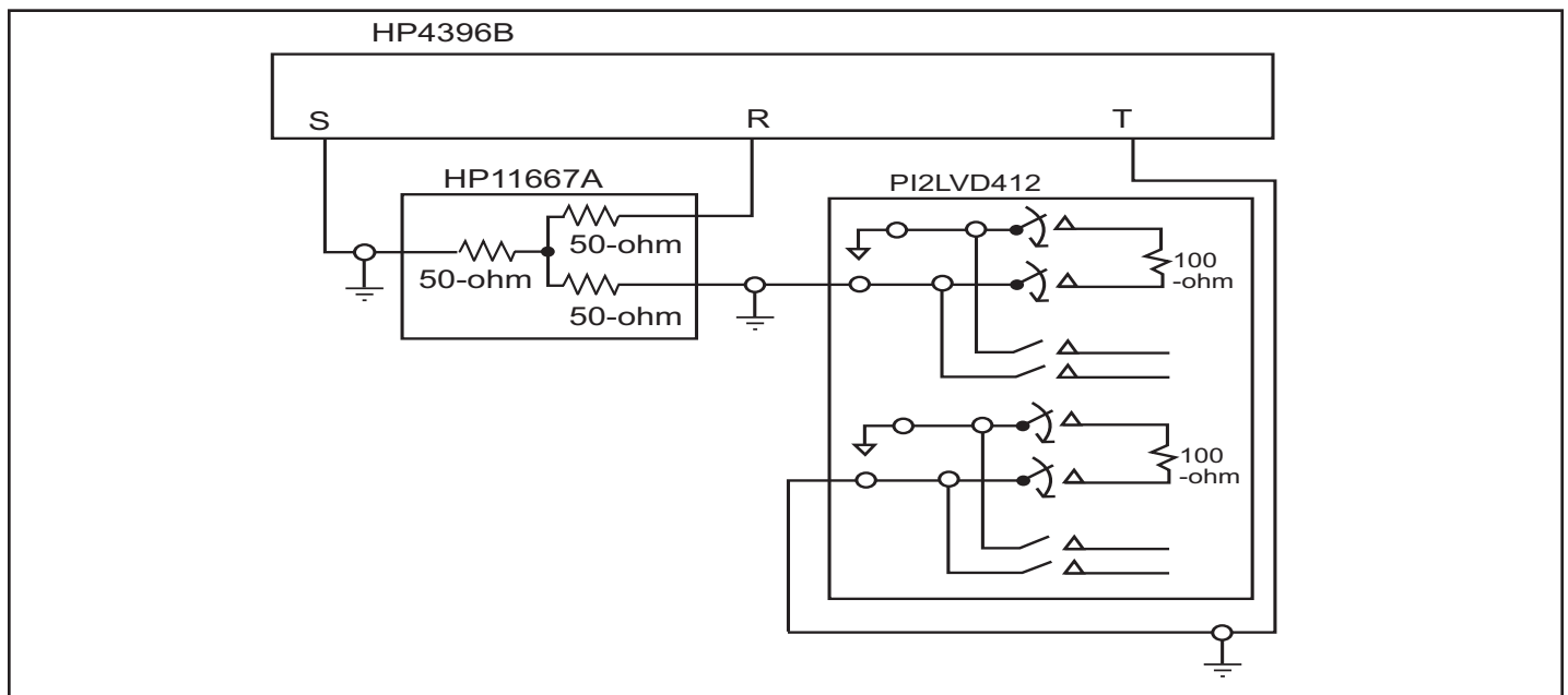
Fig 1. Crosstalk Setup
