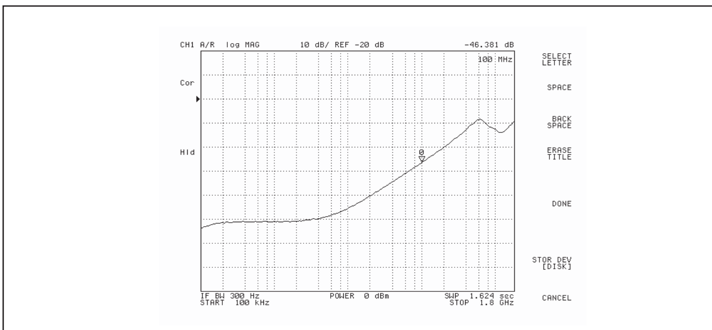
Fig 6. Off Isolation, V_{DD} = 1.8V, 25^{\circ}C
