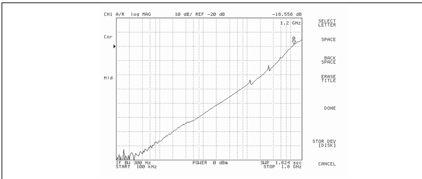
Fig 5. Crosstalk, V_{DD} = 1.8V, 25^{\circ}C
