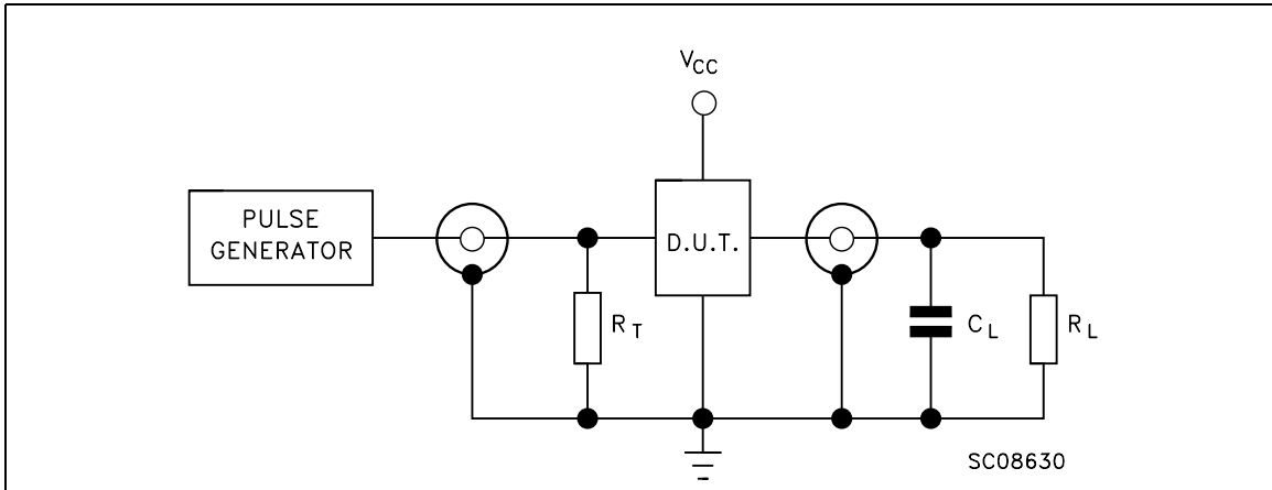
Figure 8. Test circuit
