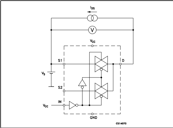
Figure 5. OFF leakage
