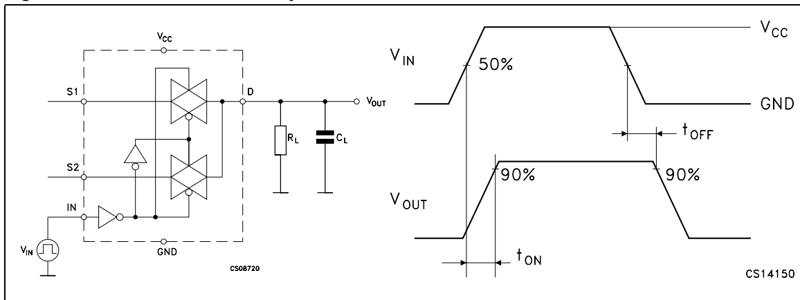
Figure 11. Turn ON, turn OFF delay time
