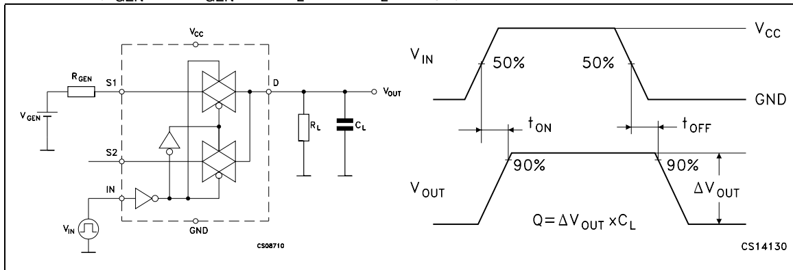
Figure 11. Turn ON, turn OFF delay time
