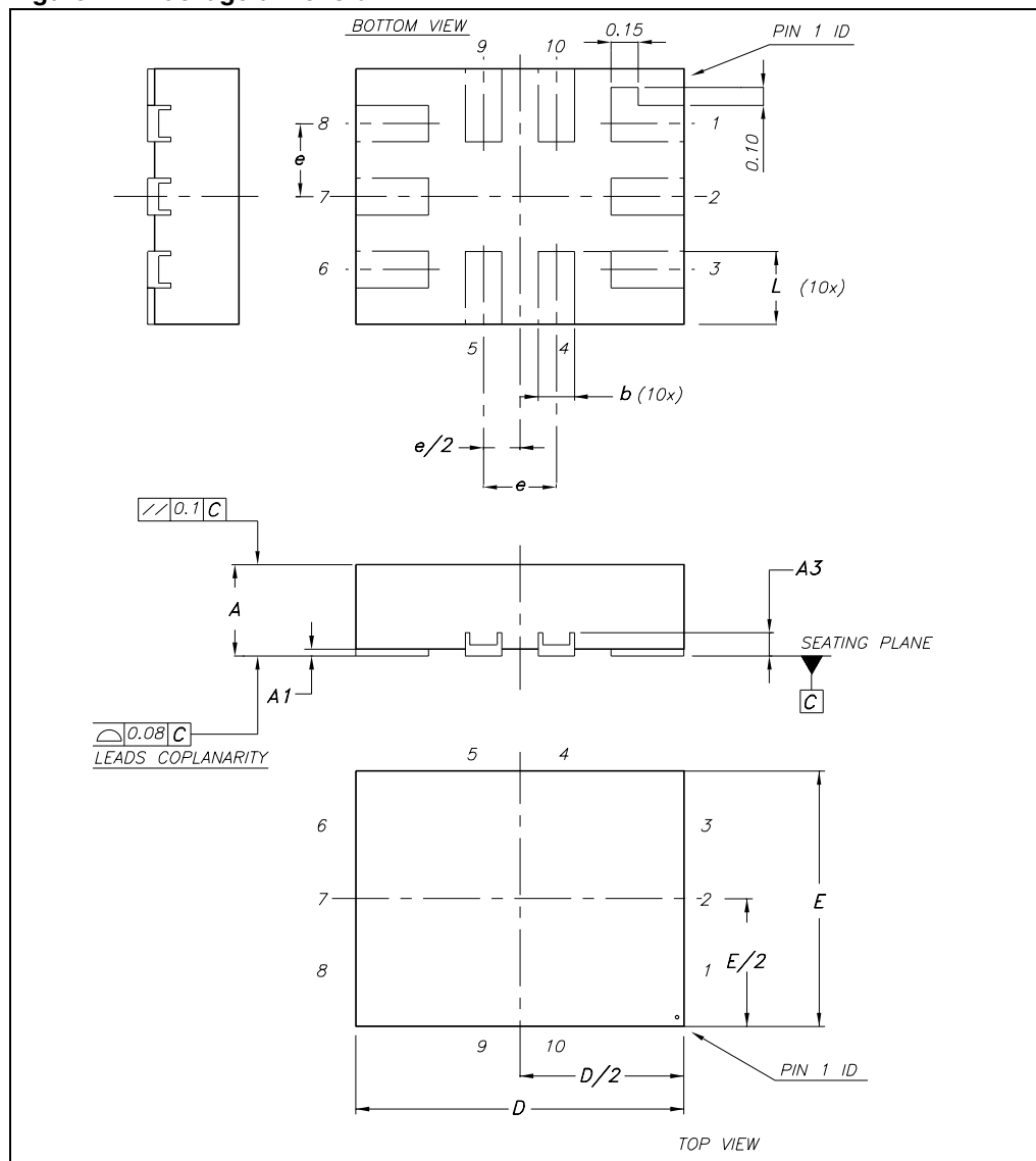
Figure 12. Package dimension
