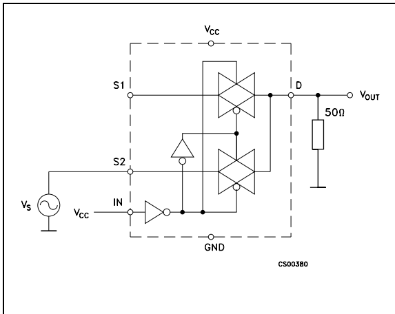
Figure 7. OFF isolation
