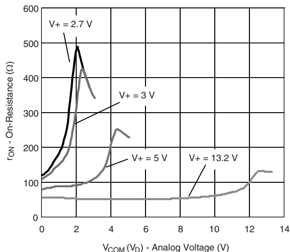
On-Resistance vs. V D (Single Supply)
