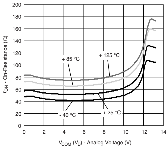
On-Resistance vs. Temperature (Single Supply)
