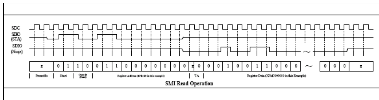
Figure 3 SMI Read Operation
