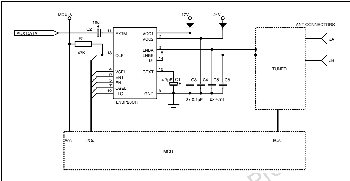
Figure 25. Two antenna ports receiver
