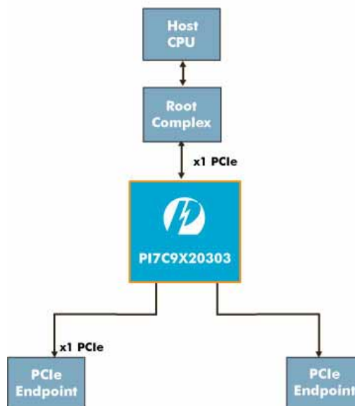
PI7C9X20303SL – Application Example
