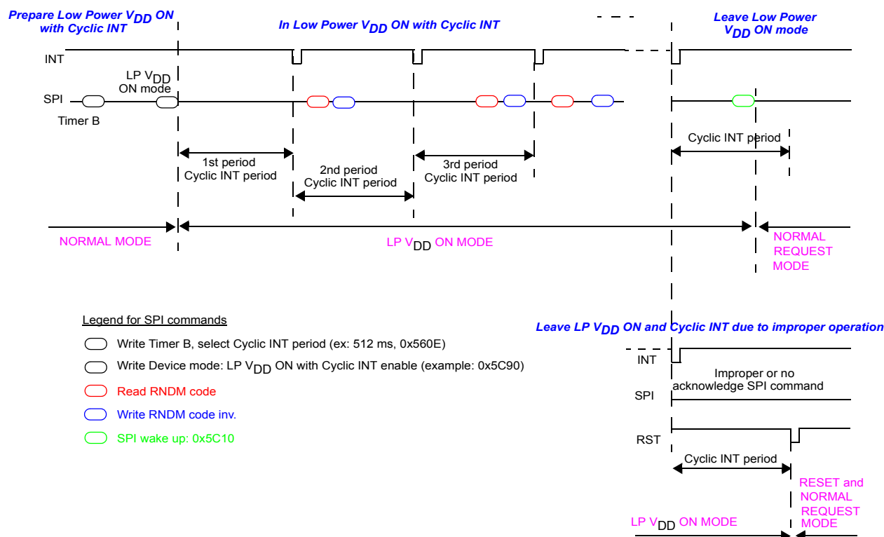
Figure 24. Cyclic Interrupt Operation
