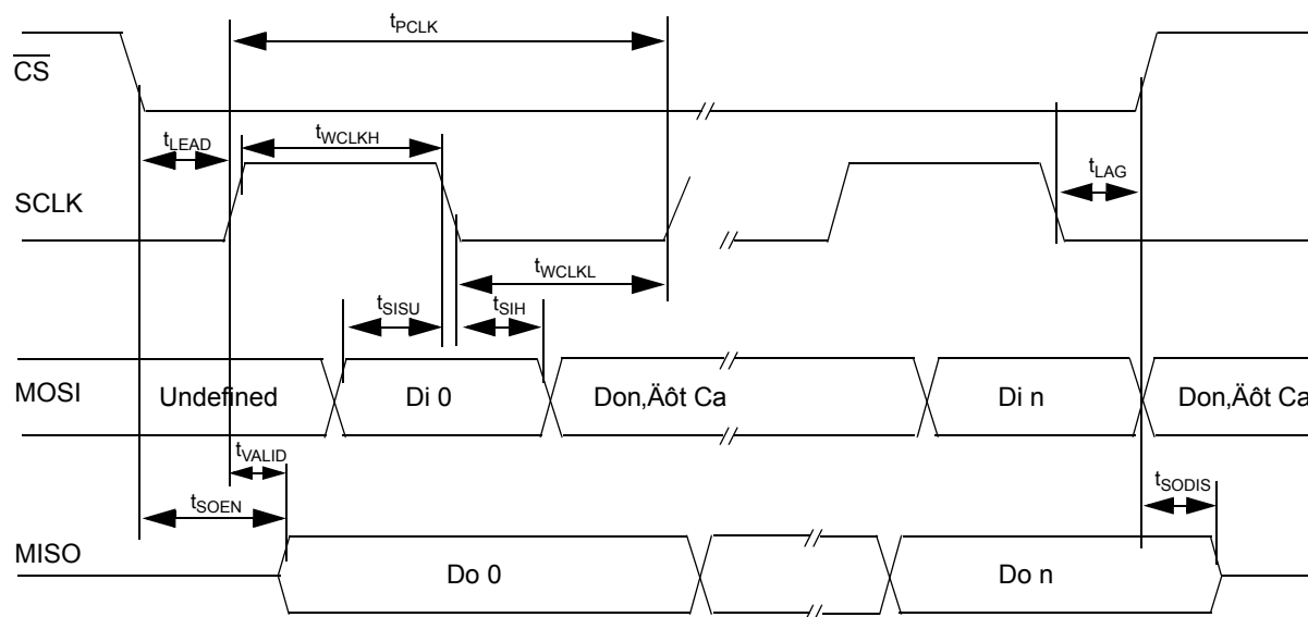
Figure 11. SPI Timings
