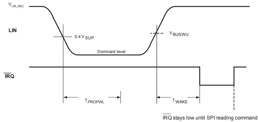
Figure 18. LIN Wake-up Low Power V DD ON Mode Timing
