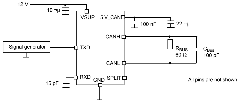
Figure 14. Test Circuit for CAN Timing Characteristics
