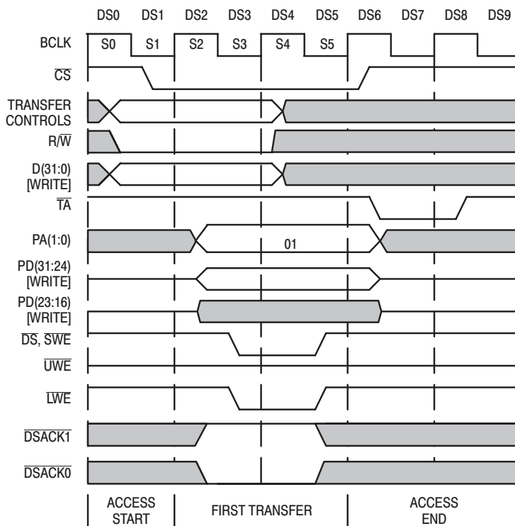
Figure 36. 8-Bit '040 WRITE to 8-Bit Peripheral Example (PA1,PA0=01)
