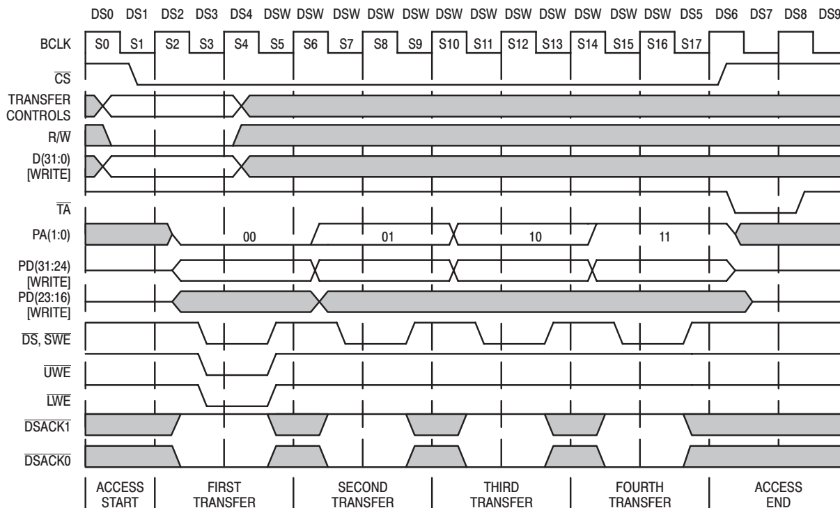
Figure 14. 32-Bit '040 WRITE to 8-Bit Peripheral Example
