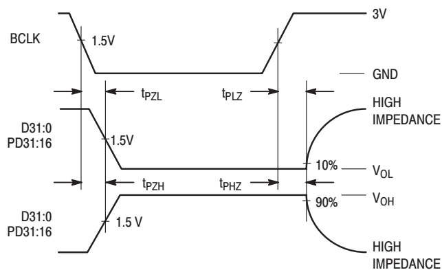
Figure 10. Enable/Disable Times
