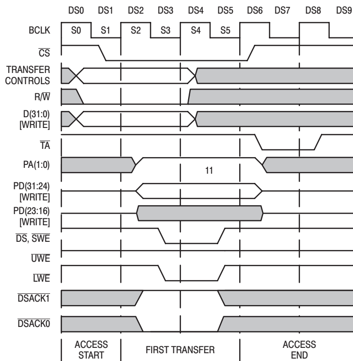
Figure 40. 8-Bit '040 WRITE to 8-Bit Peripheral Example (PA1,PA0=11)
