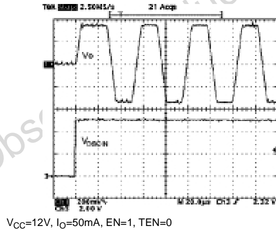
Figure 36: DSQIN Tone Enable Transient Response
