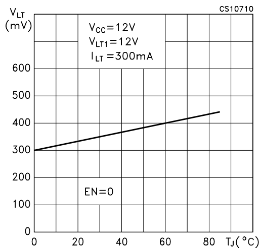
Figure 25: Loophtrough Switch Drop Voltage vs Temperature
