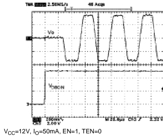
Figure 35: DSQIN Tone Enable Transient Response
