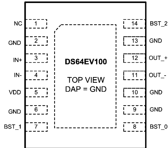
20196402 14-Pin LLP Package (3 mm x 4 mm x 0.8 mm, 0.5 mm pitch) See NS Package Number SQA14A
