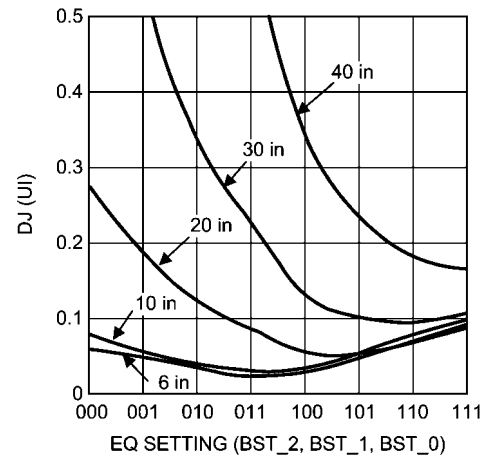
Figure 12. DJ vs. EQ Setting (6.4 Gbps)
