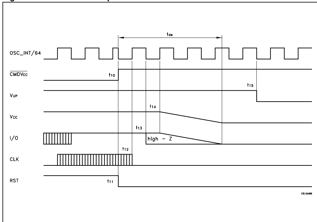
Figure 6. Deactivation sequence
