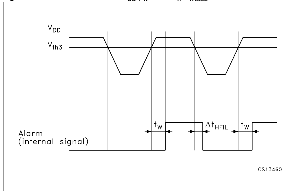
Figure 4. Alarm as a function of V_{DD} ( t_w = 10\text{ ms} ), V_{THSEL} = GND
