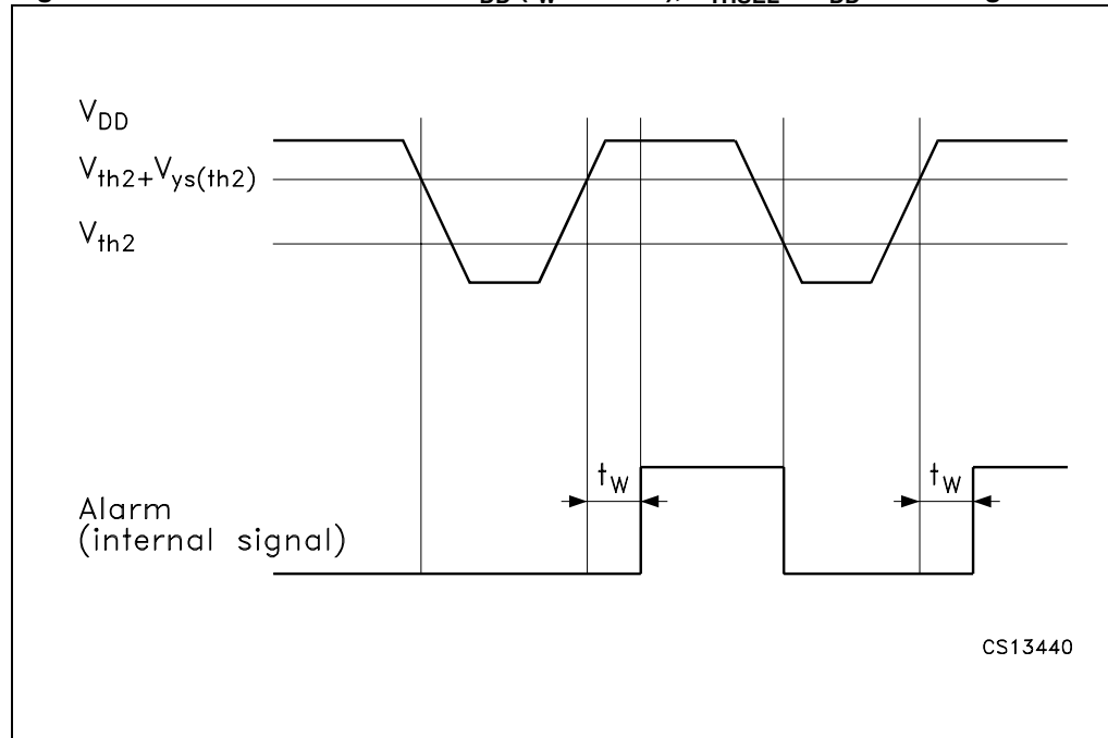
Figure 4. Alarm as a function of V_{DD} ( t_w = 10\text{ ms} ), V_{THSEL} = GND
