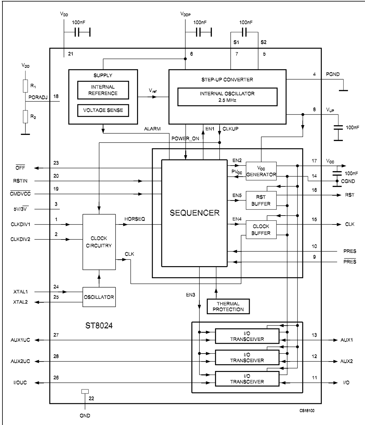
Figure 1. Block diagram
