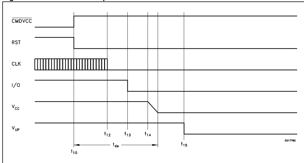
Figure 7. Deactivation sequence
