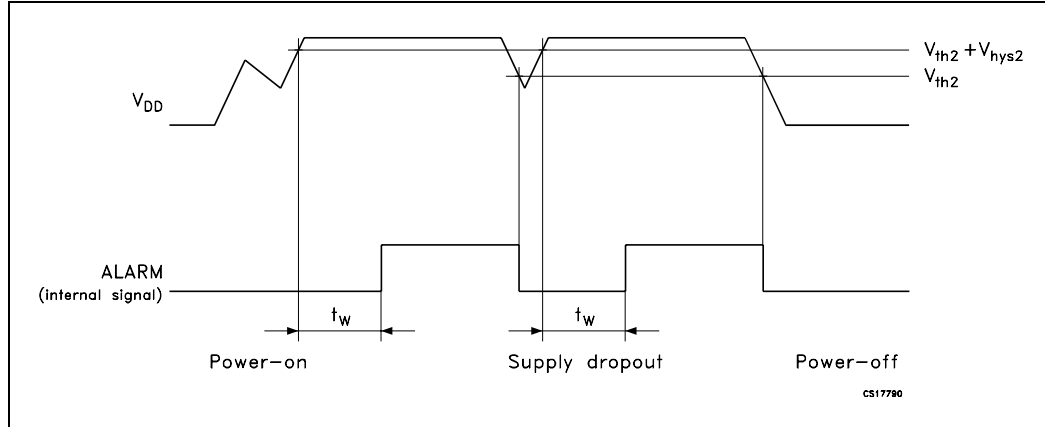
Figure 4. Voltage supervisor
