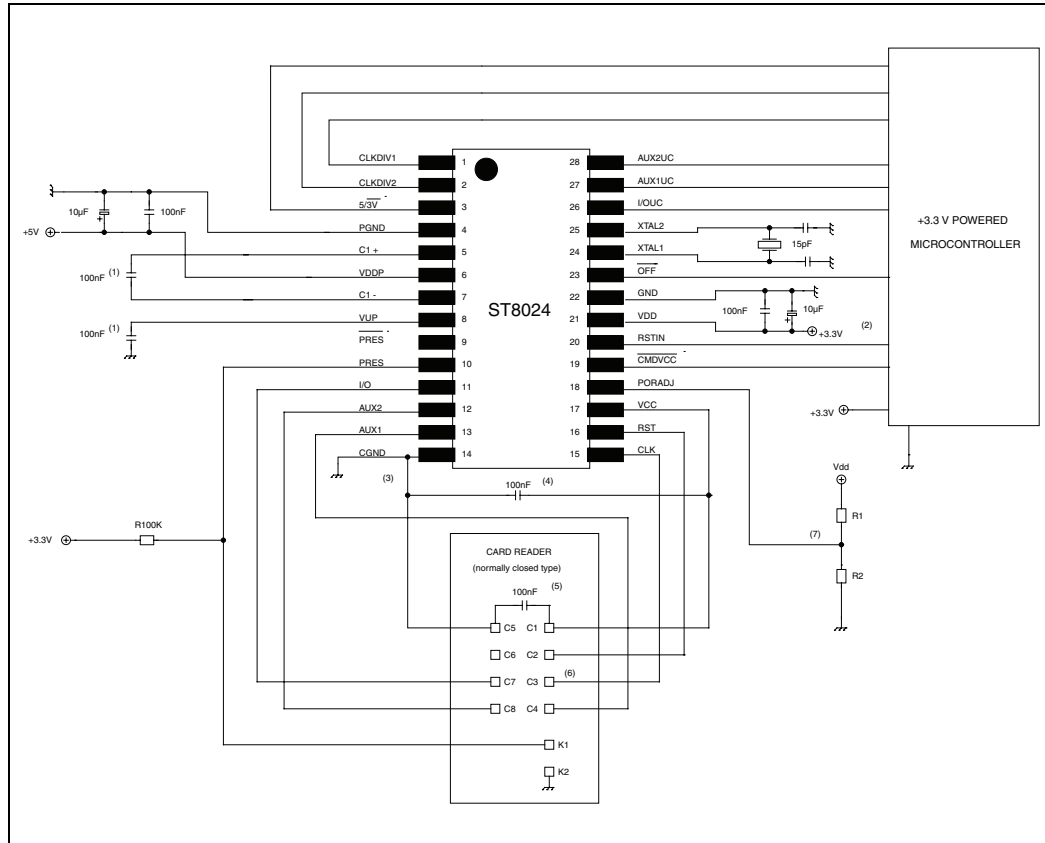
Figure 10. Application diagram
