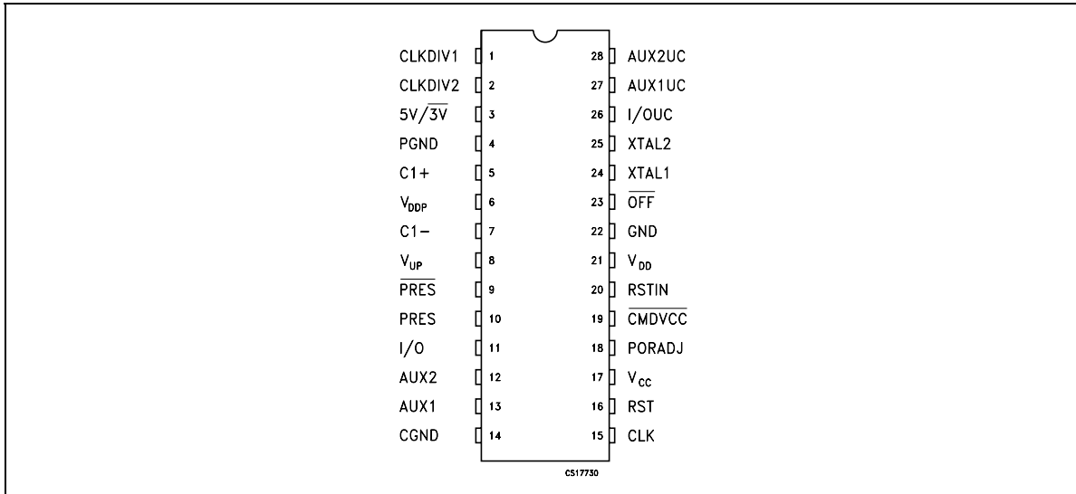
Figure 2. Pin connections
