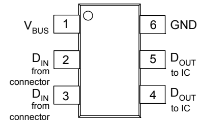
SF PACKAGE (Top View)
