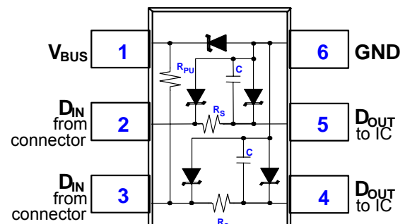
Functional Schematic with PinOut
