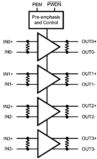
20188901 DS15BR400 Block Diagram
