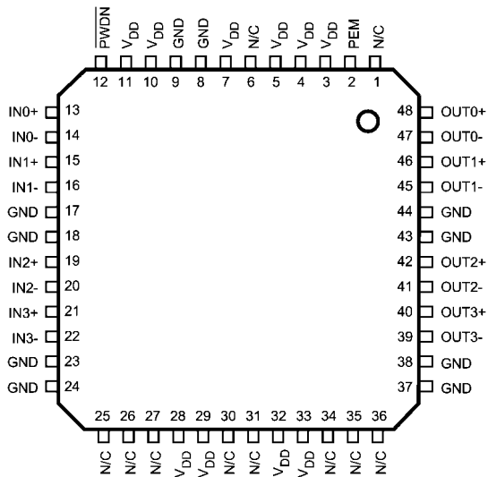
20188902 TQFP Pinout - Top View
