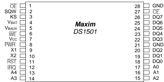
TSOP
