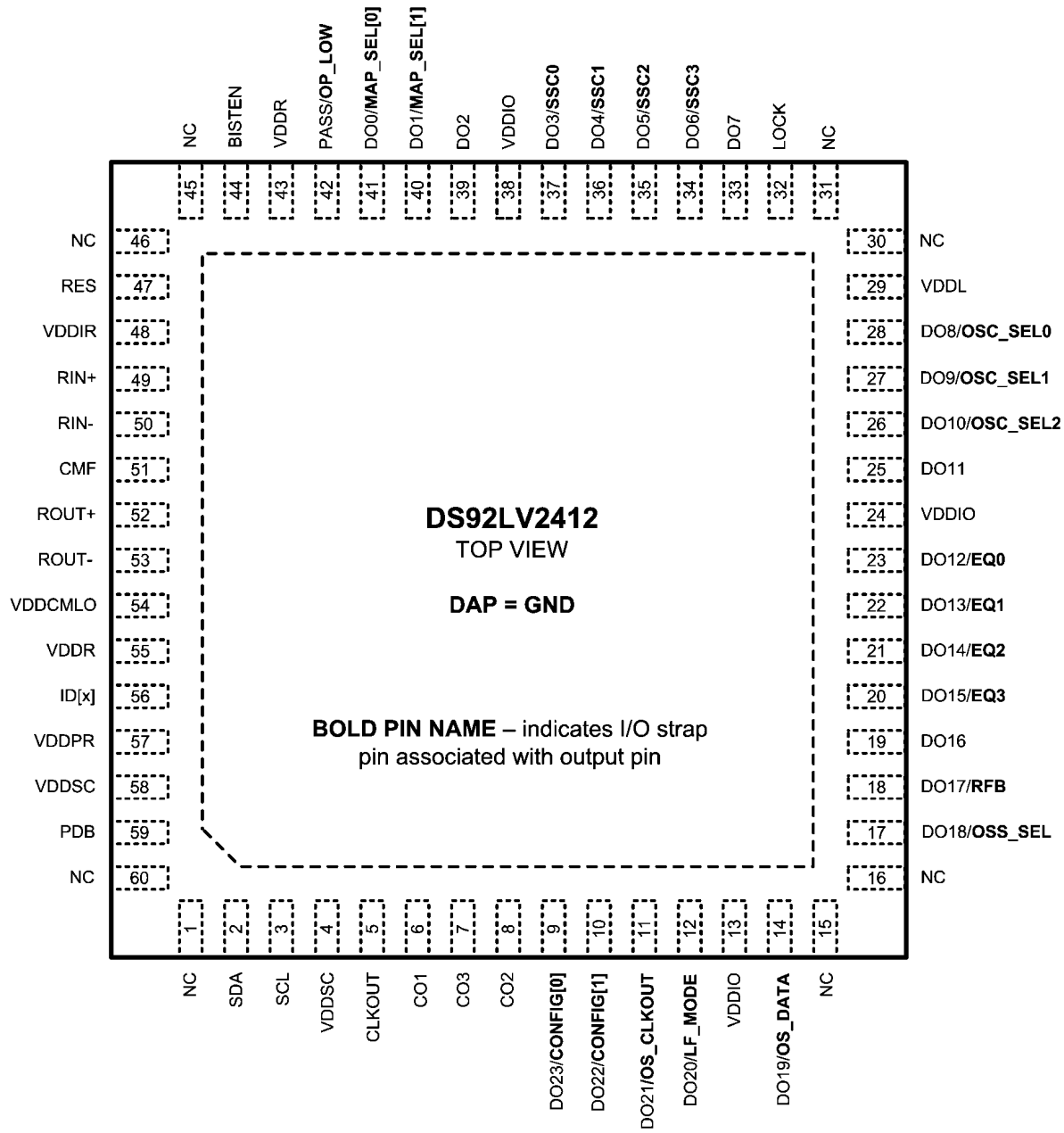
Deserializer - DS92LV2412 — Top View
