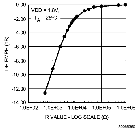
FIGURE 19. De-Emph vs. R value
