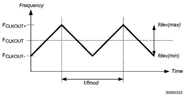
FIGURE 20. SSCG Waveform
