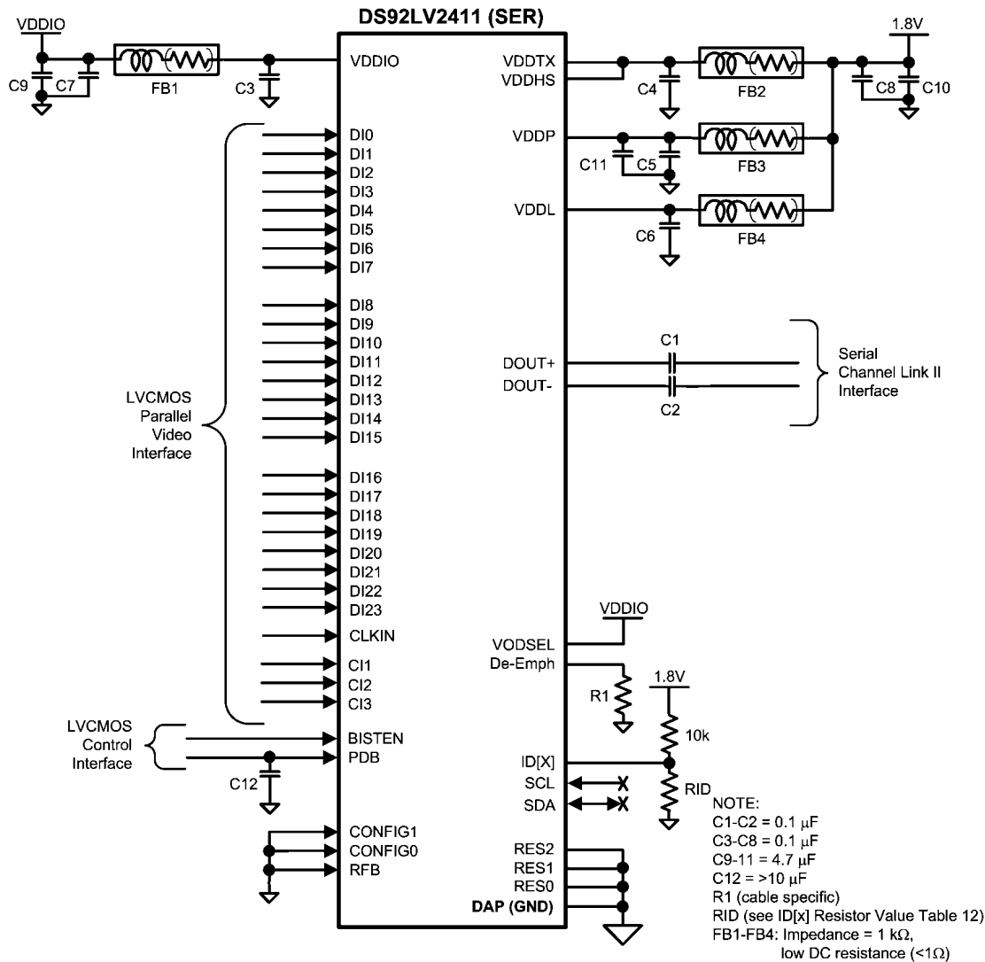
FIGURE 32. DS92LV2411 Typical Connection Diagram — Pin Control
