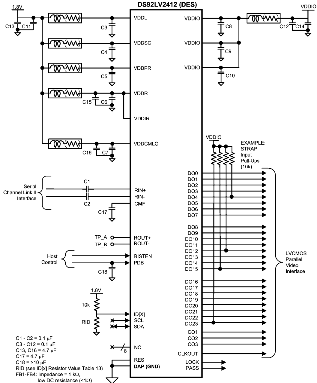
FIGURE 33. DS92LV2412 Typical Connection Diagram — Pin Control
