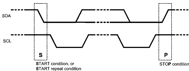
FIGURE 29. START and STOP Conditions
