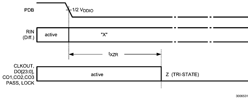
FIGURE 12. Deserializer Disable Time (OSS_SEL = 0)
