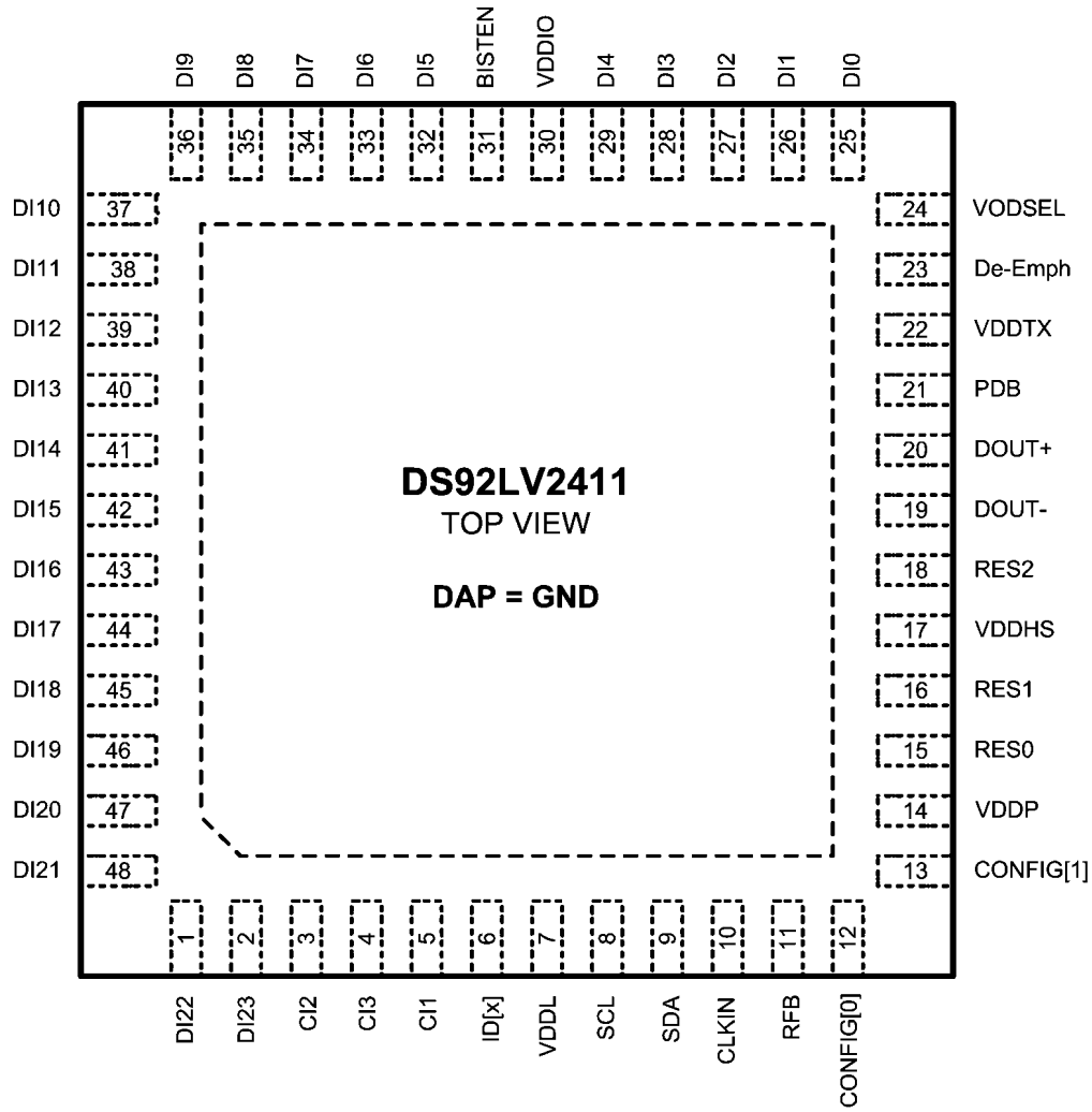
Serializer - DS92LV2411 — Top View
