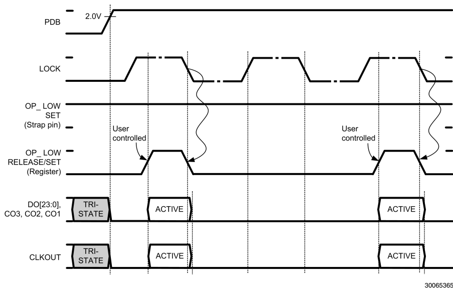
FIGURE 24. OP_LOW Auto Set
