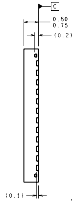
48-pin LLP Package (7.0 mm x 7.0 mm x 0.8 mm, 0.5 mm pitch) NS Package Number SQA48A
