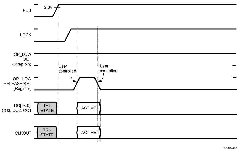
FIGURE 25. OP_LOW Manual Set/Reset
