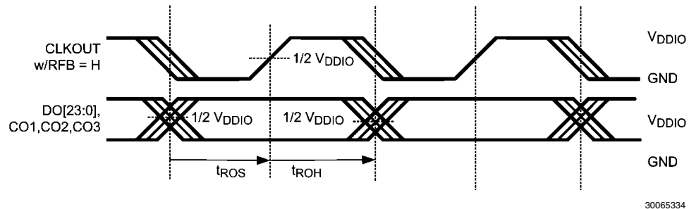
FIGURE 15. Deserializer Output Data Valid (Setup and Hold) Times with SSCG = On
