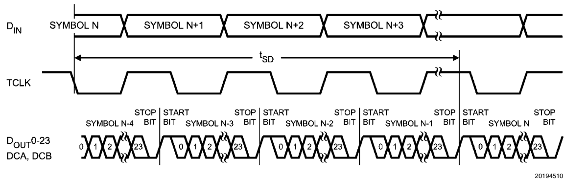
FIGURE 8. Serializer Delay
