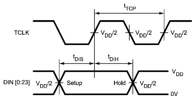
FIGURE 5. Serializer Setup/Hold Times
